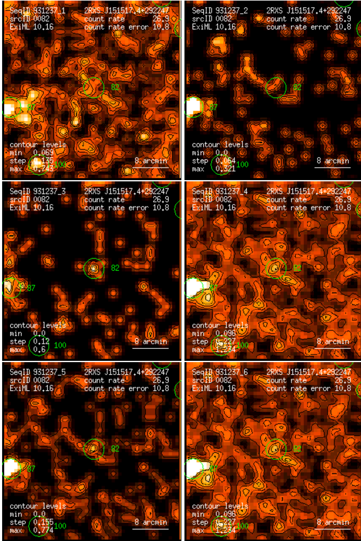
Figure 82: RASS 931237: detection 0082: band rate images, Gaussian filter: (1) PSPC channels 11 – 41, (2) 52 – 90, (3) 91 – 201, (4) 11 – 235, (5) 52 – 201, (6) 11 – 201. Broad band rates in counts/ks. Band rate contour levels in counts/ks/arcmin 2 .
