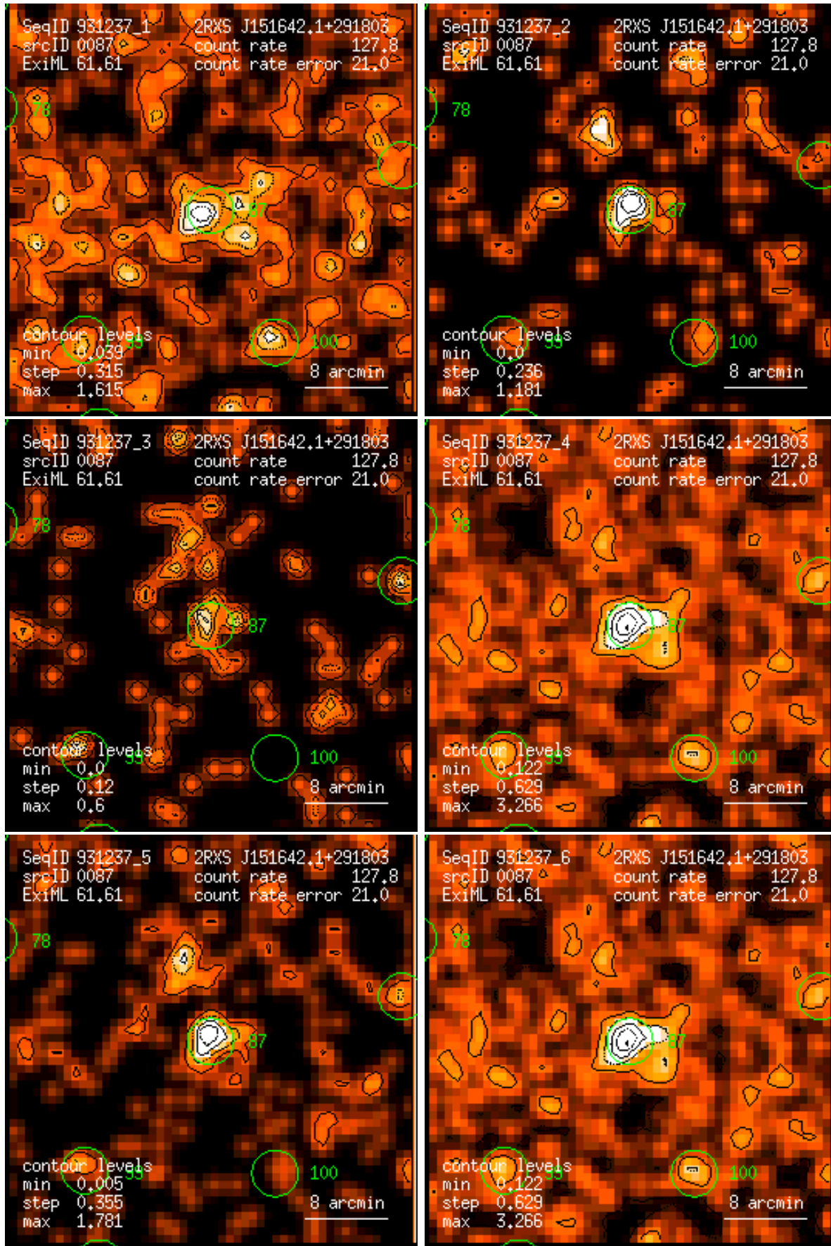
Figure 87: RASS 931237: detection 0087: band rate images, Gaussian filter: (1) PSPC channels 11 – 41, (2) 52 – 90, (3) 91 – 201, (4) 11 – 235, (5) 52 – 201, (6) 11 – 201. Broad band rates in counts/ks. Band rate contour levels in counts/ks/arcmin 2 .
