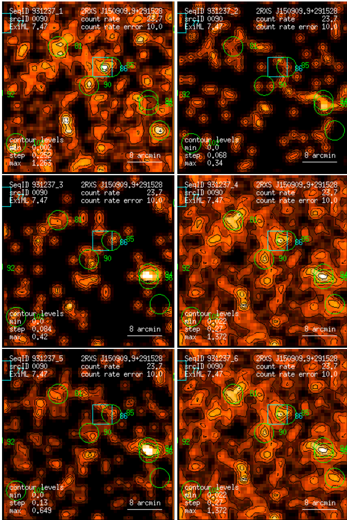
Figure 90: RASS 931237: detection 0090: band rate images, Gaussian filter: (1) PSPC channels 11 – 41, (2) 52 – 90, (3) 91 – 201, (4) 11 – 235, (5) 52 – 201, (6) 11 – 201. Broad band rates in counts/ks. Band rate contour levels in counts/ks/arcmin 2 .
