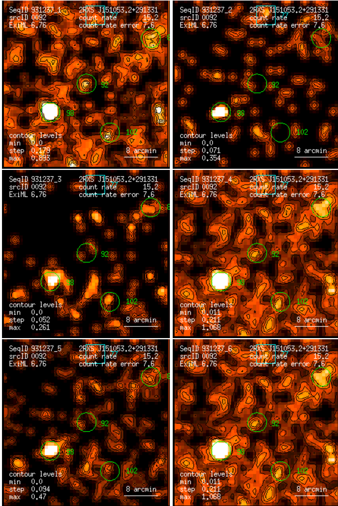
Figure 92: RASS 931237: detection 0092: band rate images, Gaussian filter: (1) PSPC channels 11 – 41, (2) 52 – 90, (3) 91 – 201, (4) 11 – 235, (5) 52 – 201, (6) 11 – 201. Broad band rates in counts/ks. Band rate contour levels in counts/ks/arcmin 2 .
