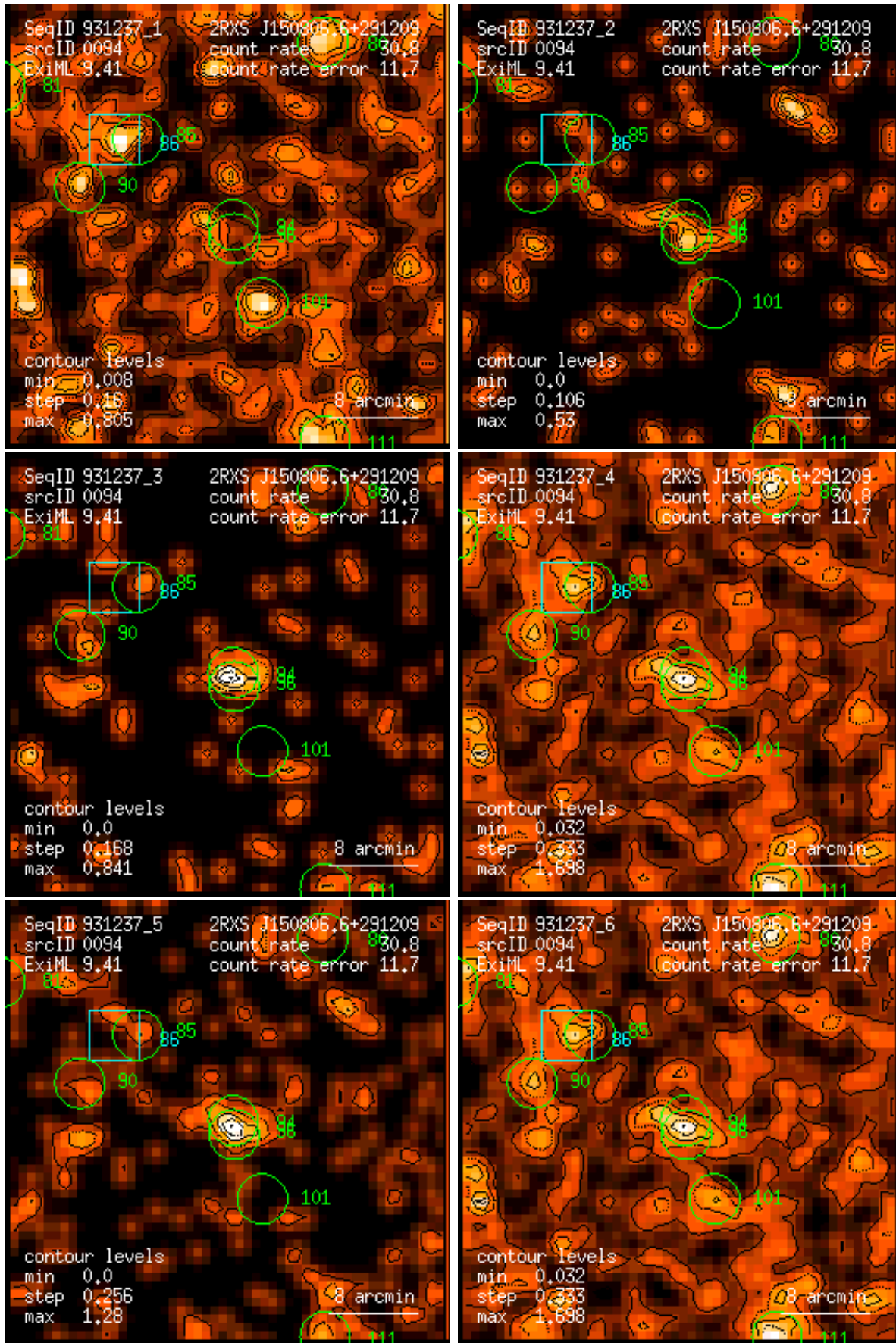
Figure 94: RASS 931237: detection 0094: band rate images, Gaussian filter: (1) PSPC channels 11 – 41, (2) 52 – 90, (3) 91 – 201, (4) 11 – 235, (5) 52 – 201, (6) 11 – 201. Broad band rates in counts/ks. Band rate contour levels in counts/ks/arcmin 2 .
