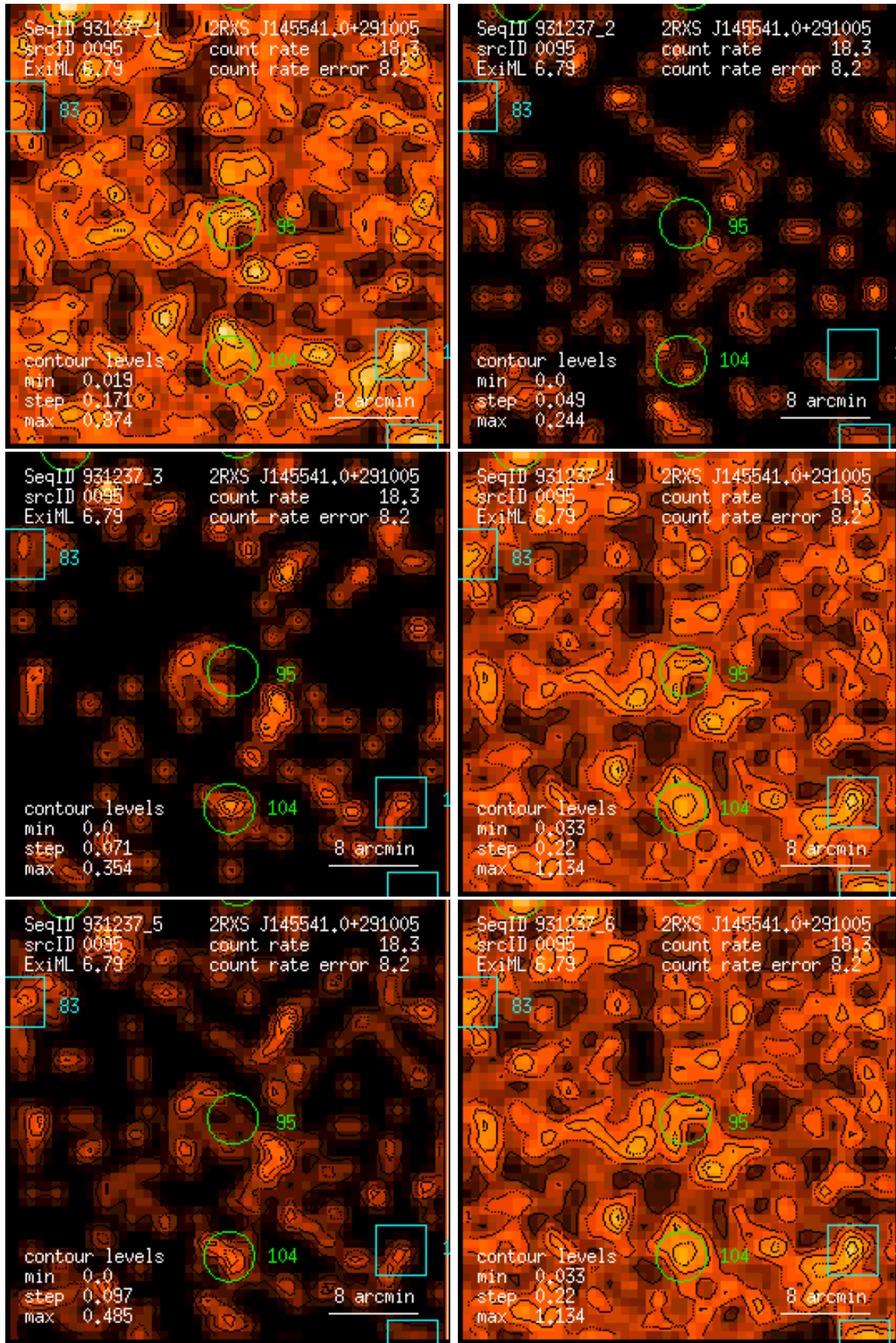
Figure 95: RASS 931237: detection 0095: band rate images, Gaussian filter: (1) PSPC channels 11 – 41, (2) 52 – 90, (3) 91 – 201, (4) 11 – 235, (5) 52 – 201, (6) 11 – 201. Broad band rates in counts/ks. Band rate contour levels in counts/ks/arcmin 2 .
