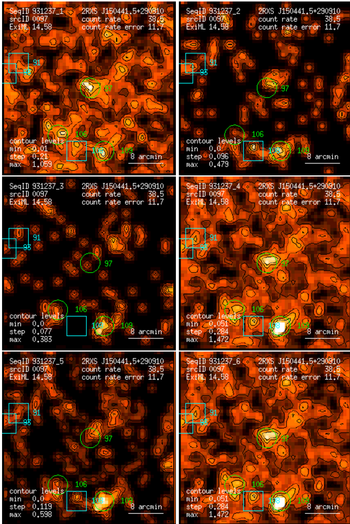
Figure 97: RASS 931237: detection 0097: band rate images, Gaussian filter: (1) PSPC channels 11 – 41, (2) 52 – 90, (3) 91 – 201, (4) 11 – 235, (5) 52 – 201, (6) 11 – 201. Broad band rates in counts/ks. Band rate contour levels in counts/ks/arcmin 2 .
