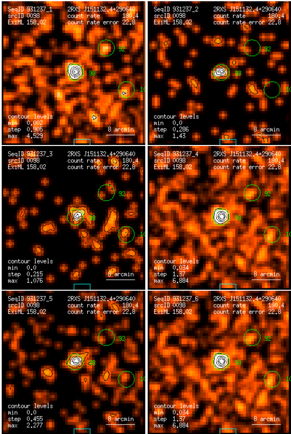
Figure 98: RASS 931237: detection 0098: band rate images, Gaussian filter: (1) PSPC channels 11 – 41, (2) 52 – 90, (3) 91 – 201, (4) 11 – 235, (5) 52 – 201, (6) 11 – 201. Broad band rates in counts/ks. Band rate contour levels in counts/ks/arcmin 2 .
