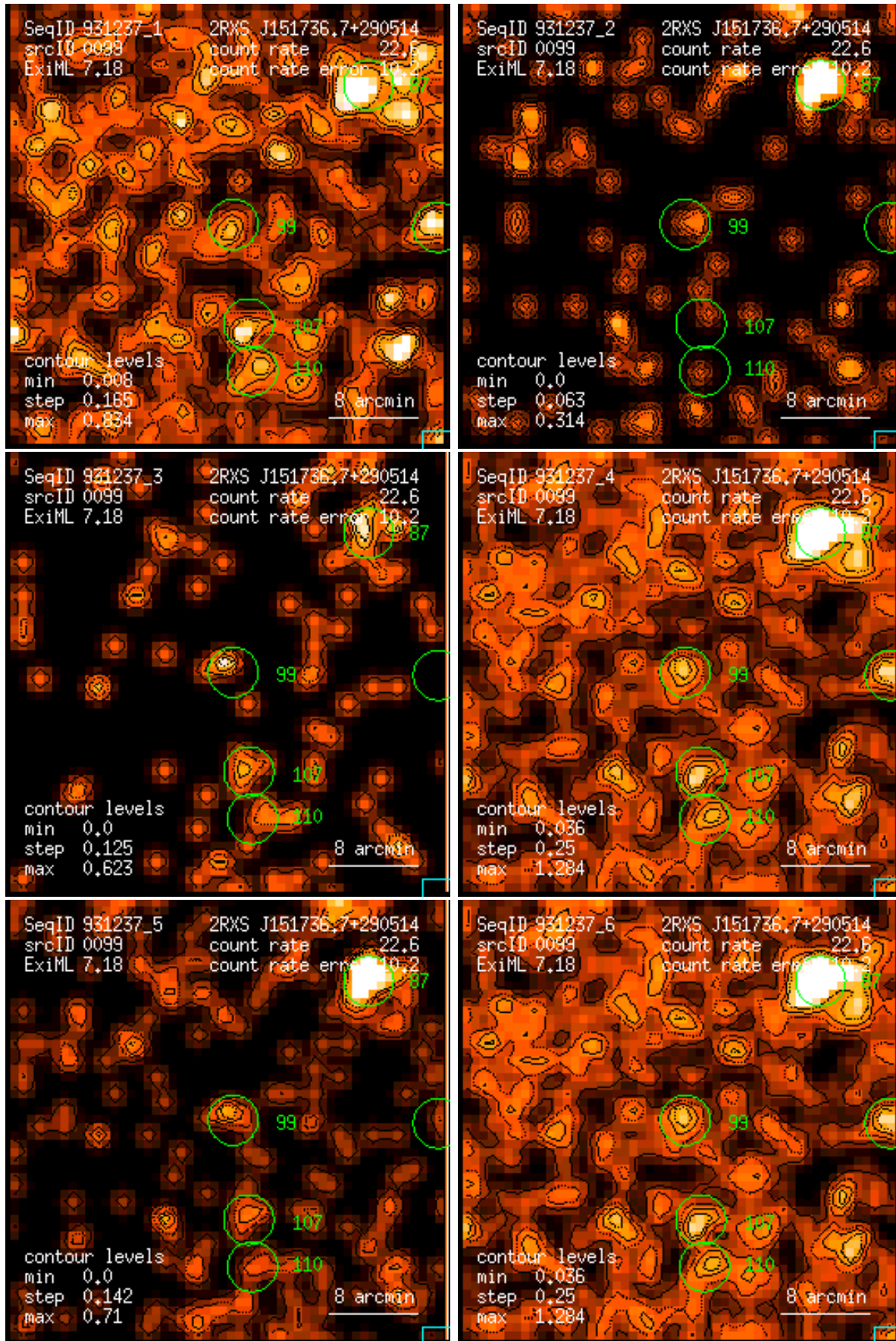
Figure 99: RASS 931237: detection 0099: band rate images, Gaussian filter: (1) PSPC channels 11 – 41, (2) 52 – 90, (3) 91 – 201, (4) 11 – 235, (5) 52 – 201, (6) 11 – 201. Broad band rates in counts/ks. Band rate contour levels in counts/ks/arcmin 2 .
