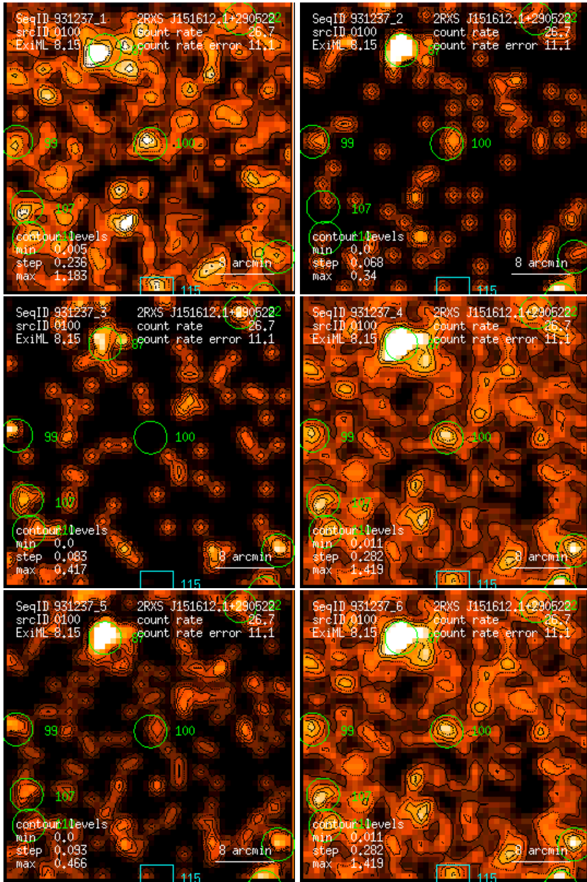
Figure 100: RASS 931237: detection 0100: band rate images, Gaussian filter: (1) PSPC channels 11 – 41, (2) 52 – 90, (3) 91 – 201, (4) 11 – 235, (5) 52 – 201, (6) 11 – 201. Broad band rates in counts/ks. Band rate contour levels in counts/ks/arcmin 2 .
