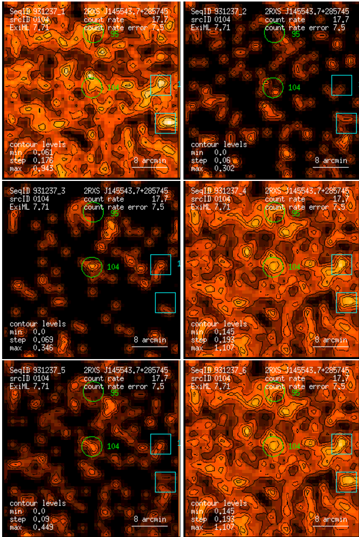
Figure 104: RASS 931237: detection 0104: band rate images, Gaussian filter: (1) PSPC channels 11 – 41, (2) 52 – 90, (3) 91 – 201, (4) 11 – 235, (5) 52 – 201, (6) 11 – 201. Broad band rates in counts/ks. Band rate contour levels in counts/ks/arcmin 2 .
