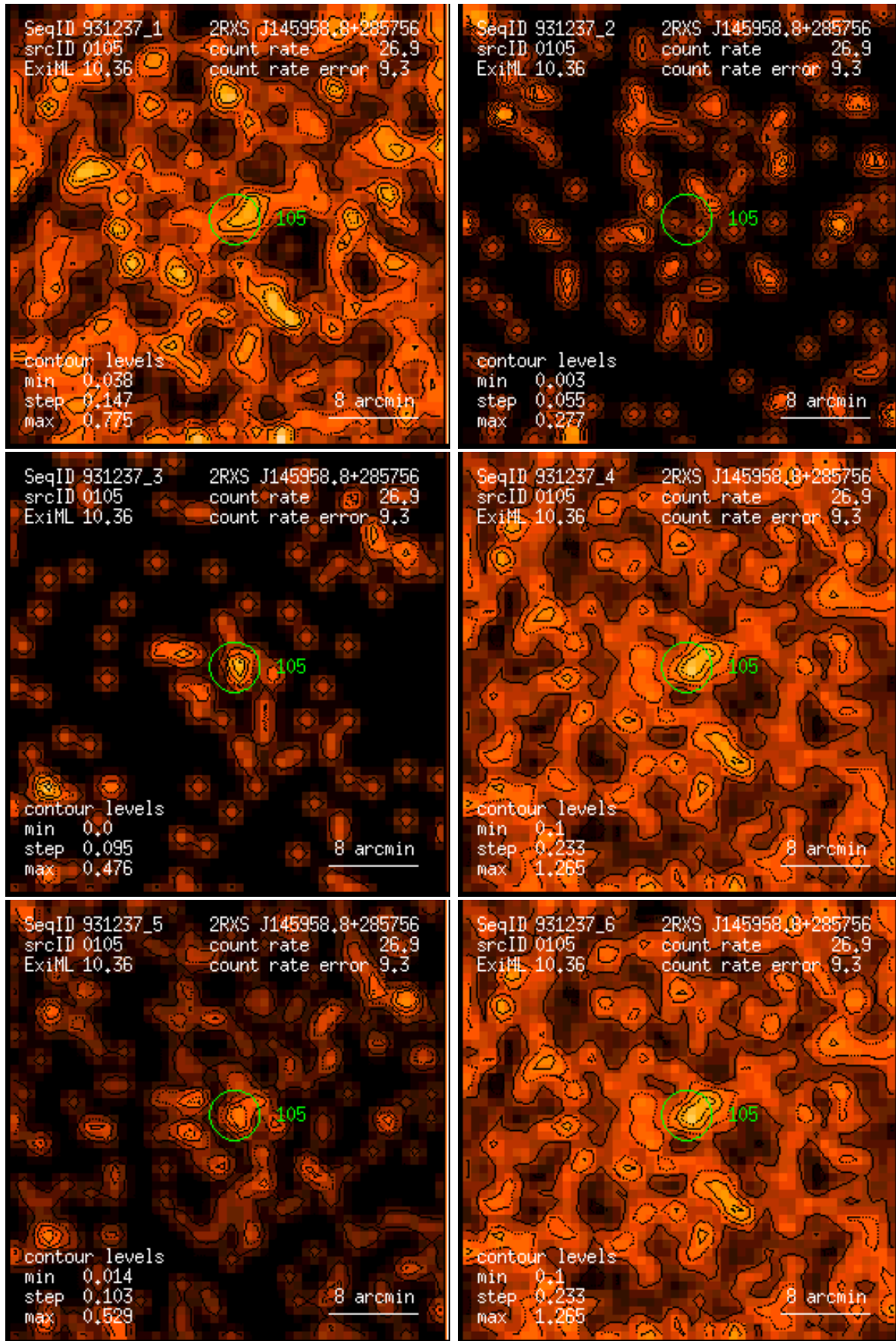
Figure 105: RASS 931237: detection 0105: band rate images, Gaussian filter: (1) PSPC channels 11 – 41, (2) 52 – 90, (3) 91 – 201, (4) 11 – 235, (5) 52 – 201, (6) 11 – 201. Broad band rates in counts/ks. Band rate contour levels in counts/ks/arcmin 2 .
