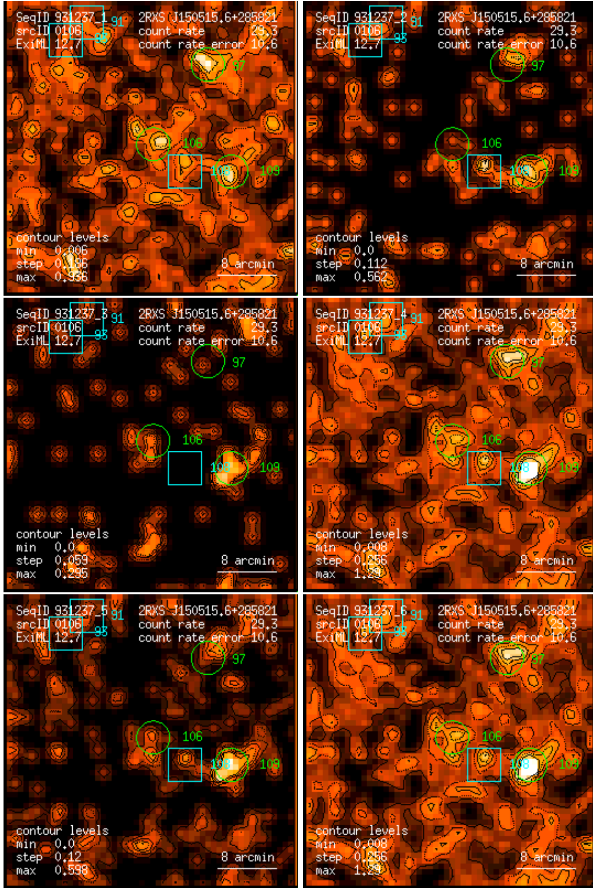
Figure 106: RASS 931237: detection 0106: band rate images, Gaussian filter: (1) PSPC channels 11 – 41, (2) 52 – 90, (3) 91 – 201, (4) 11 – 235, (5) 52 – 201, (6) 11 – 201. Broad band rates in counts/ks. Band rate contour levels in counts/ks/arcmin 2 .
