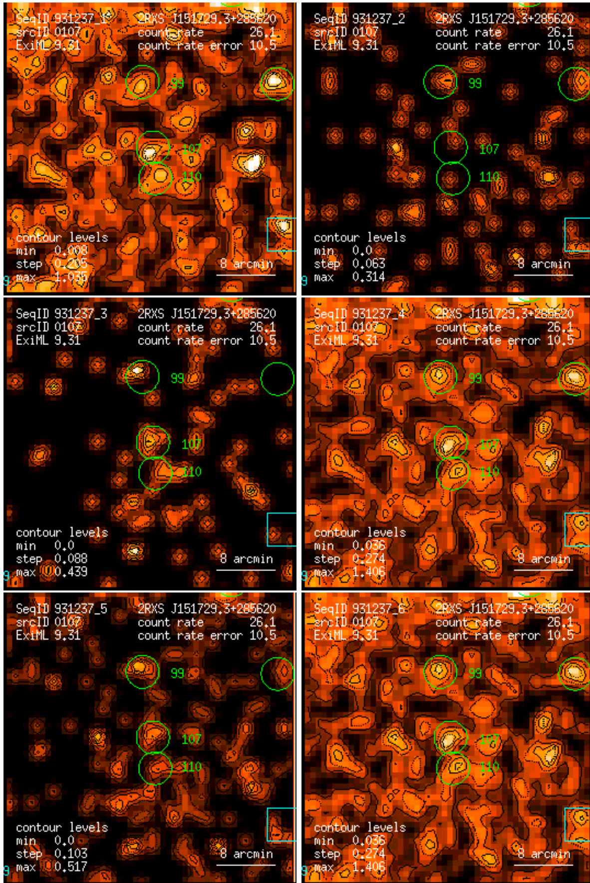
Figure 107: RASS 931237: detection 0107: band rate images, Gaussian filter: (1) PSPC channels 11 – 41, (2) 52 – 90, (3) 91 – 201, (4) 11 – 235, (5) 52 – 201, (6) 11 – 201. Broad band rates in counts/ks. Band rate contour levels in counts/ks/arcmin 2 .
