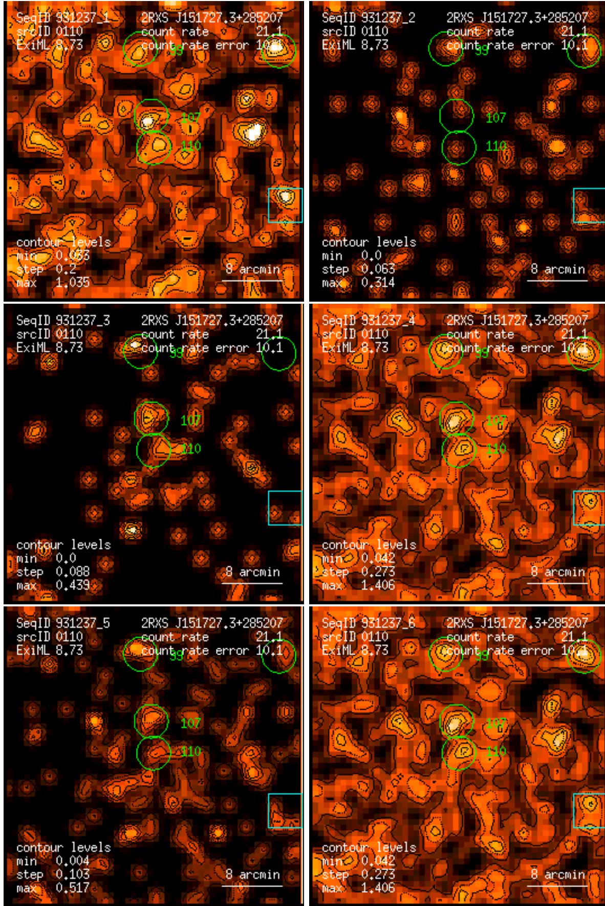
Figure 110: RASS 931237: detection 0110: band rate images, Gaussian filter: (1) PSPC channels 11 – 41, (2) 52 – 90, (3) 91 – 201, (4) 11 – 235, (5) 52 – 201, (6) 11 – 201. Broad band rates in counts/ks. Band rate contour levels in counts/ks/arcmin 2 .
