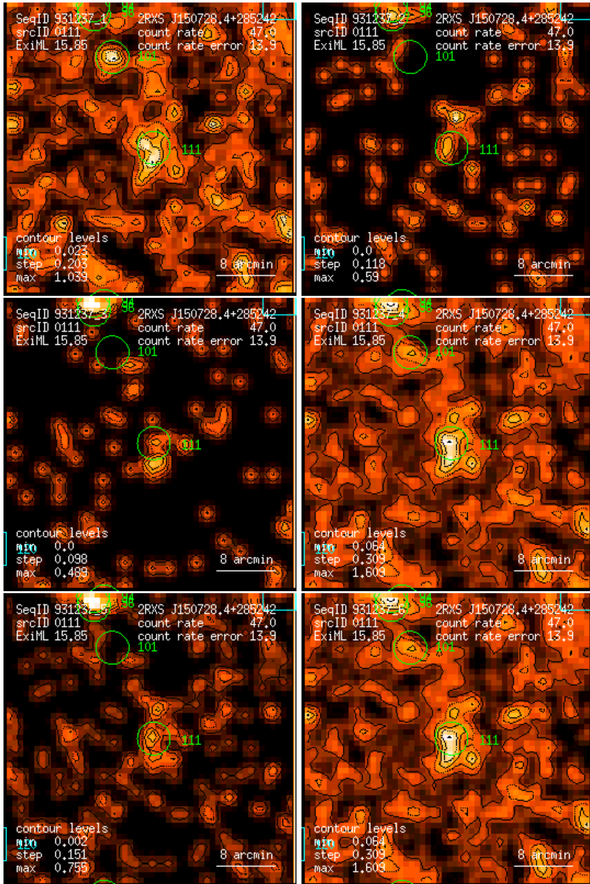
Figure 111: RASS 931237: detection 0111: band rate images, Gaussian filter: (1) PSPC channels 11 – 41, (2) 52 – 90, (3) 91 – 201, (4) 11 – 235, (5) 52 – 201, (6) 11 – 201. Broad band rates in counts/ks. Band rate contour levels in counts/ks/arcmin 2 .
