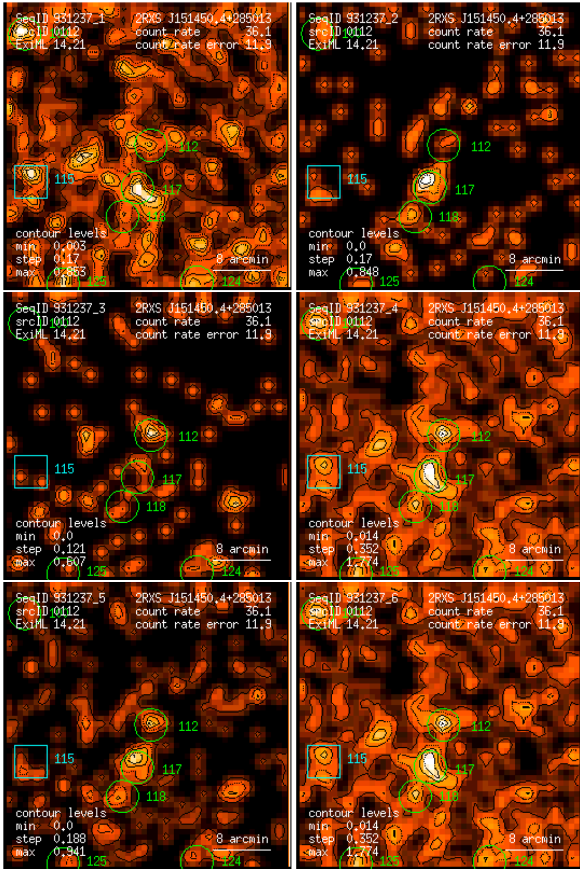
Figure 112: RASS 931237: detection 0112: band rate images, Gaussian filter: (1) PSPC channels 11 – 41, (2) 52 – 90, (3) 91 – 201, (4) 11 – 235, (5) 52 – 201, (6) 11 – 201. Broad band rates in counts/ks. Band rate contour levels in counts/ks/arcmin 2 .
