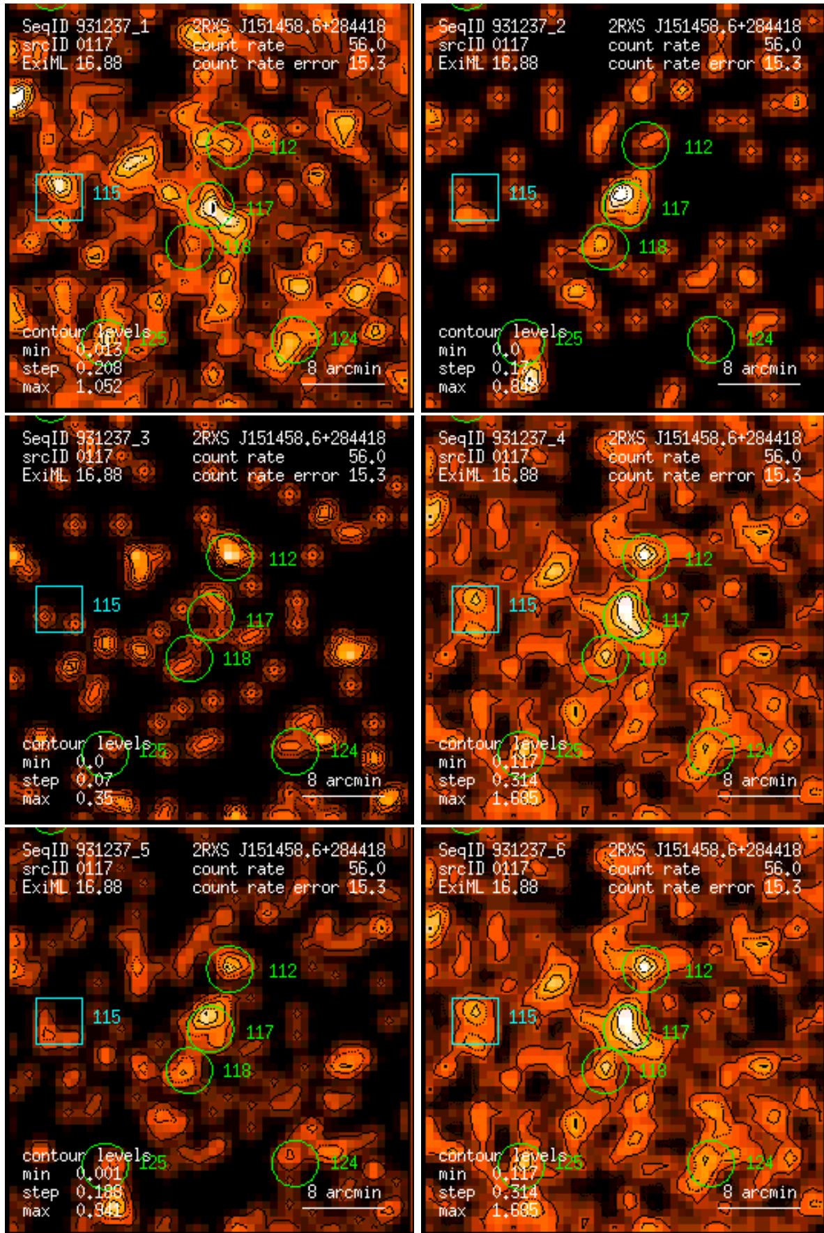
Figure 117: RASS 931237: detection 0117: band rate images, Gaussian filter: (1) PSPC channels 11 – 41, (2) 52 – 90, (3) 91 – 201, (4) 11 – 235, (5) 52 – 201, (6) 11 – 201. Broad band rates in counts/ks. Band rate contour levels in counts/ks/arcmin 2 .
