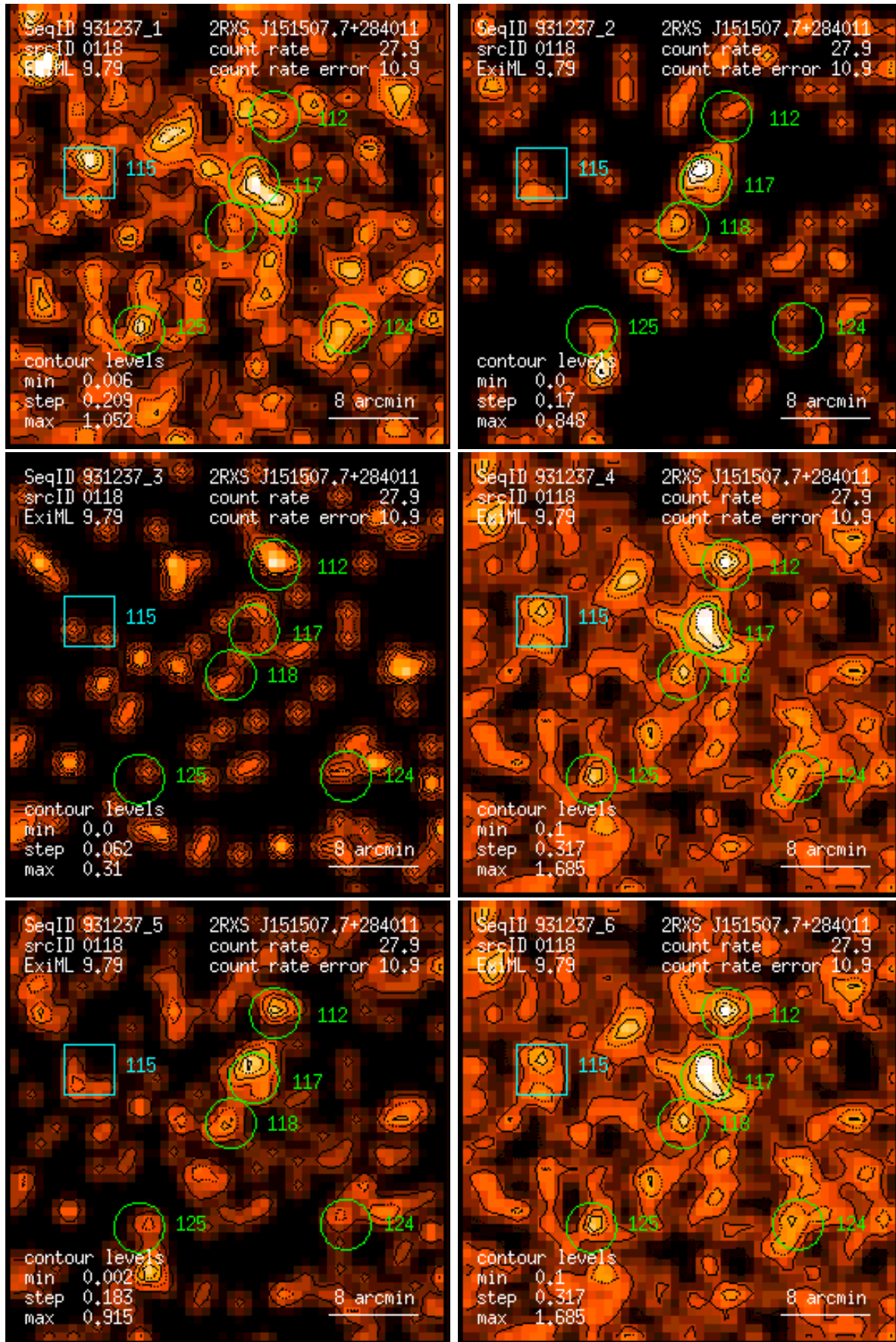
Figure 118: RASS 931237: detection 0118: band rate images, Gaussian filter: (1) PSPC channels 11 – 41, (2) 52 – 90, (3) 91 – 201, (4) 11 – 235, (5) 52 – 201, (6) 11 – 201. Broad band rates in counts/ks. Band rate contour levels in counts/ks/arcmin 2 .
