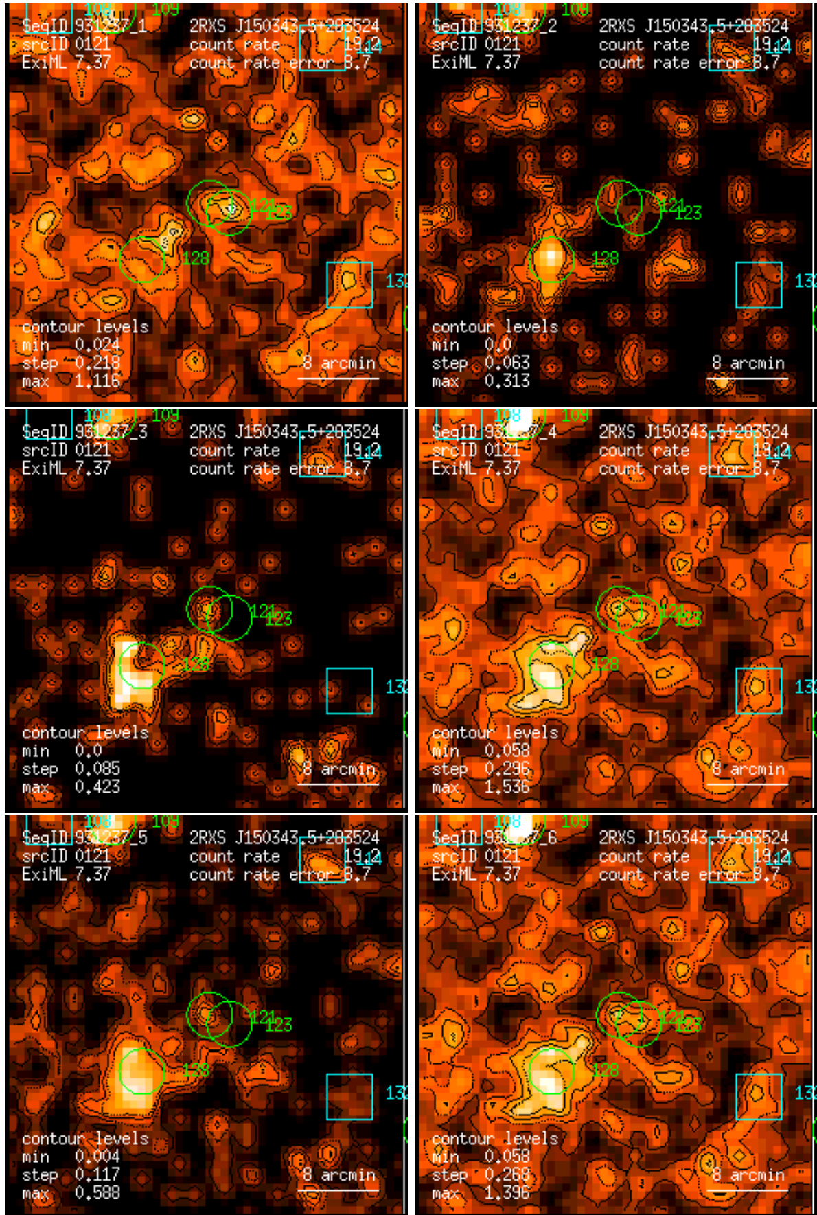
Figure 121: RASS 931237: detection 0121: band rate images, Gaussian filter: (1) PSPC channels 11 – 41, (2) 52 – 90, (3) 91 – 201, (4) 11 – 235, (5) 52 – 201, (6) 11 – 201. Broad band rates in counts/ks. Band rate contour levels in counts/ks/arcmin 2 .
