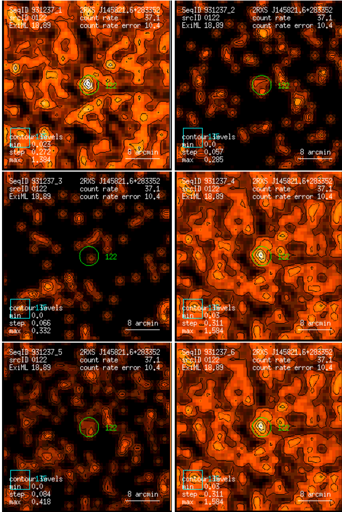
Figure 122: RASS 931237: detection 0122: band rate images, Gaussian filter: (1) PSPC channels 11 – 41, (2) 52 – 90, (3) 91 – 201, (4) 11 – 235, (5) 52 – 201, (6) 11 – 201. Broad band rates in counts/ks. Band rate contour levels in counts/ks/arcmin 2 .
