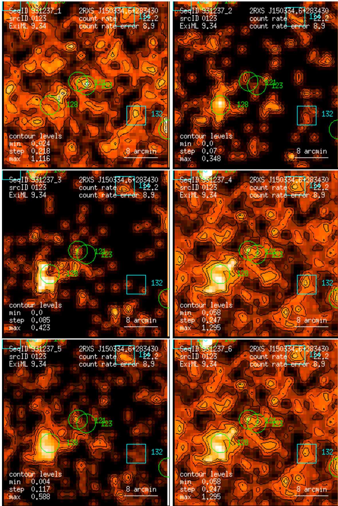
Figure 123: RASS 931237: detection 0123: band rate images, Gaussian filter: (1) PSPC channels 11 – 41, (2) 52 – 90, (3) 91 – 201, (4) 11 – 235, (5) 52 – 201, (6) 11 – 201. Broad band rates in counts/ks. Band rate contour levels in counts/ks/arcmin 2 .
