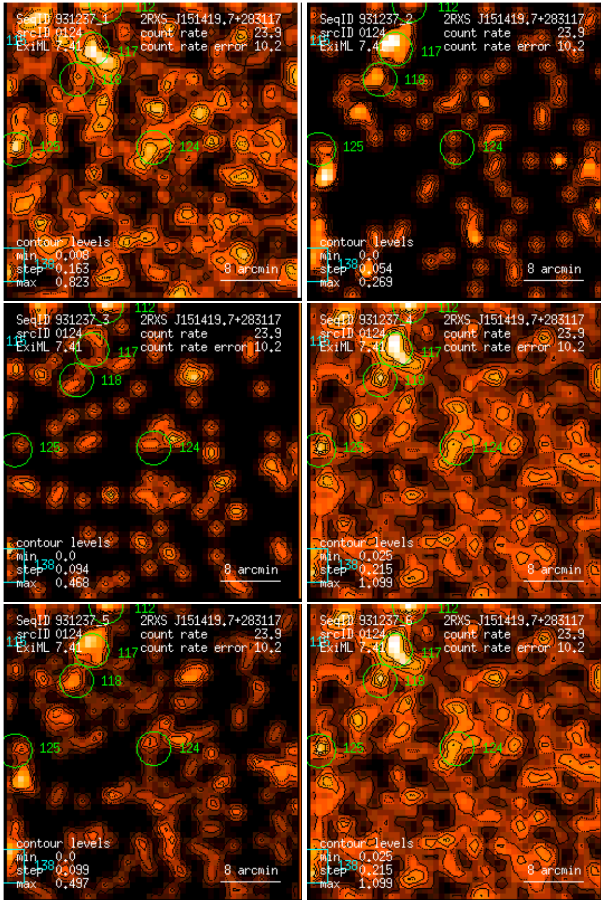
Figure 124: RASS 931237: detection 0124: band rate images, Gaussian filter: (1) PSPC channels 11 – 41, (2) 52 – 90, (3) 91 – 201, (4) 11 – 235, (5) 52 – 201, (6) 11 – 201. Broad band rates in counts/ks. Band rate contour levels in counts/ks/arcmin 2 .
