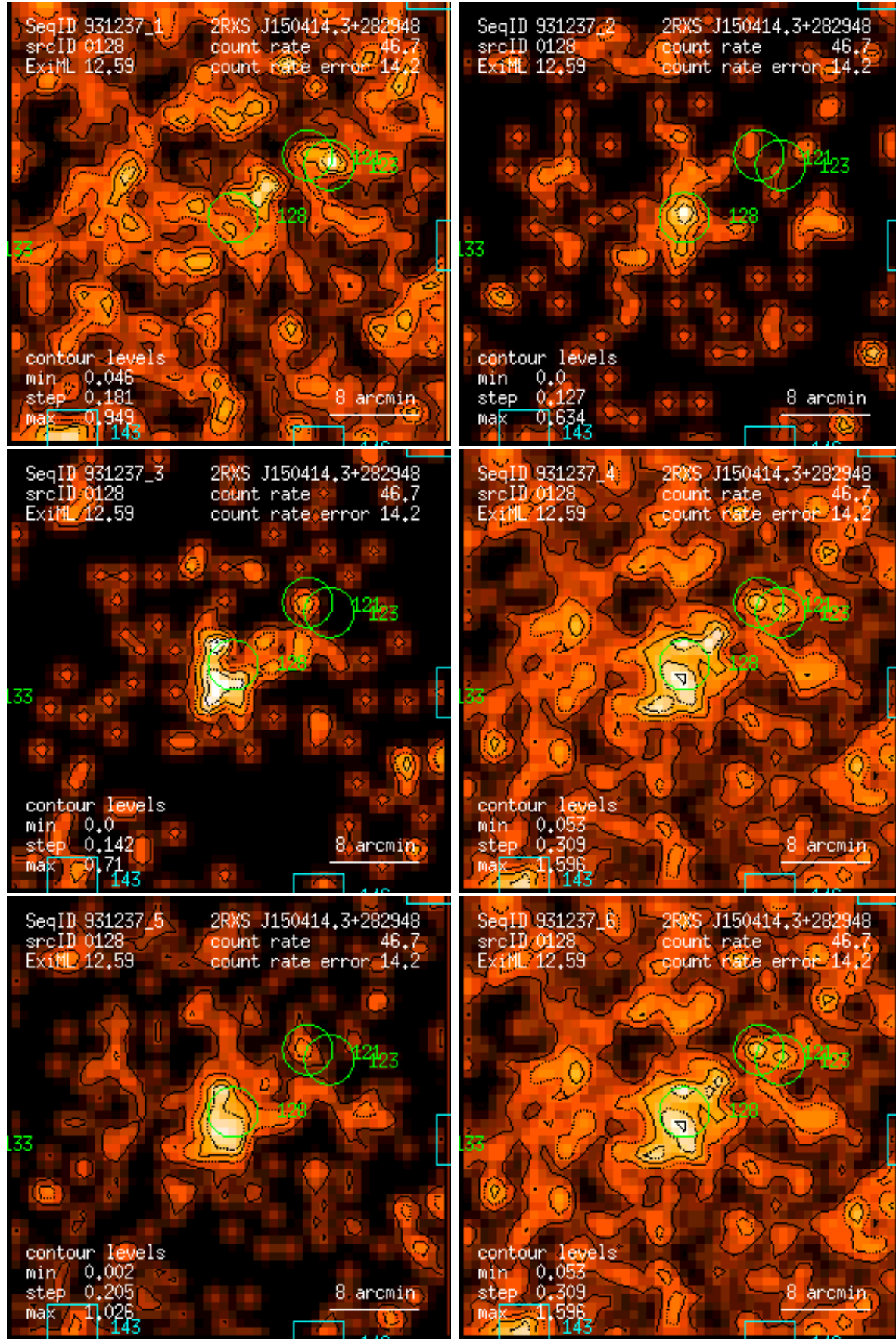
Figure 128: RASS 931237: detection 0128: band rate images, Gaussian filter: (1) PSPC channels 11 – 41, (2) 52 – 90, (3) 91 – 201, (4) 11 – 235, (5) 52 – 201, (6) 11 – 201. Broad band rates in counts/ks. Band rate contour levels in counts/ks/arcmin 2 .
