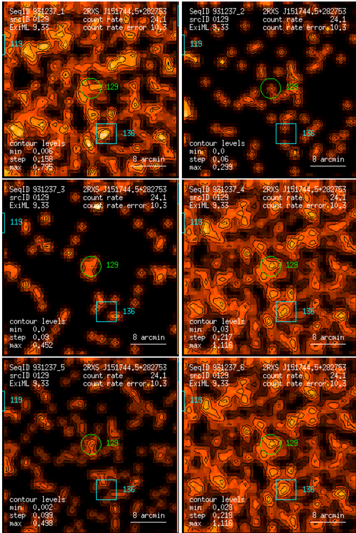
Figure 129: RASS 931237: detection 0129: band rate images, Gaussian filter: (1) PSPC channels 11 – 41, (2) 52 – 90, (3) 91 – 201, (4) 11 – 235, (5) 52 – 201, (6) 11 – 201. Broad band rates in counts/ks. Band rate contour levels in counts/ks/arcmin 2 .
