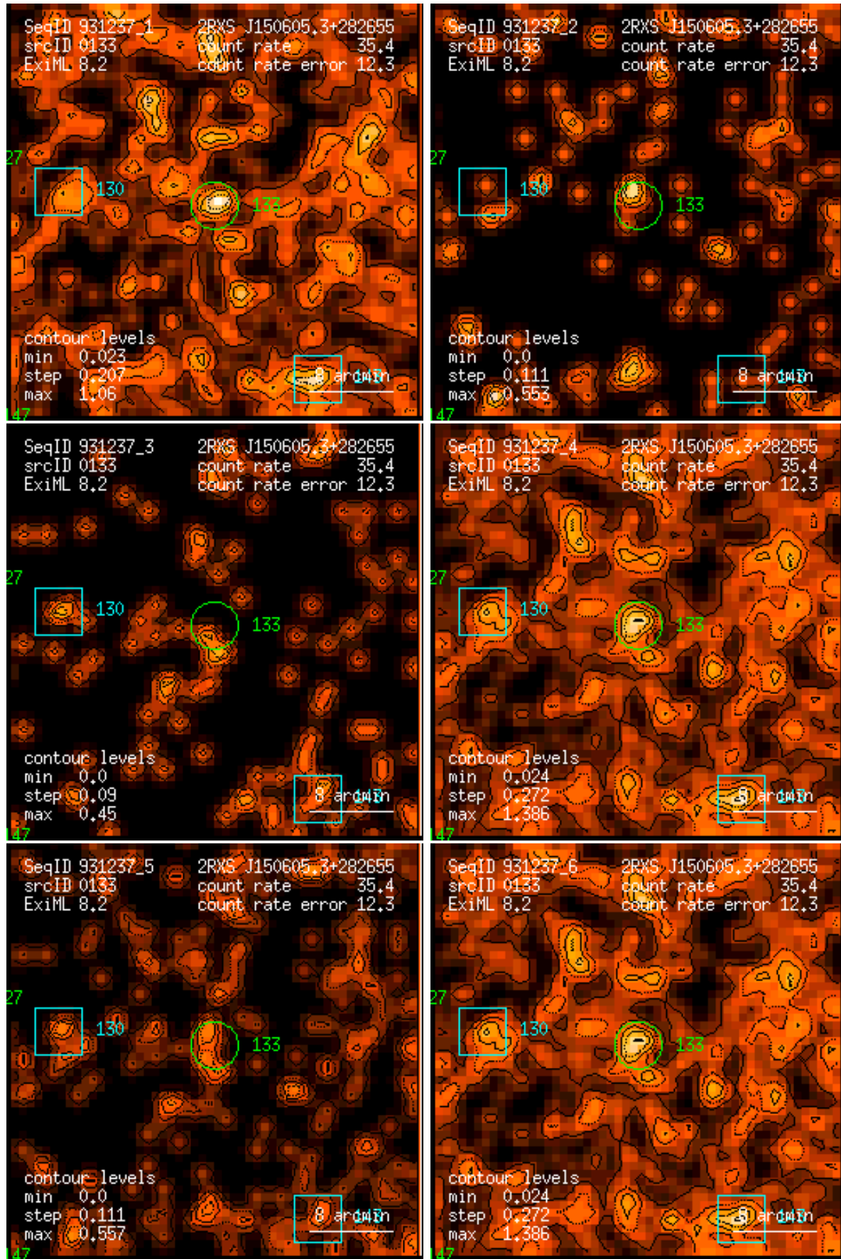
Figure 133: RASS 931237: detection 0133: band rate images, Gaussian filter: (1) PSPC channels 11 – 41, (2) 52 – 90, (3) 91 – 201, (4) 11 – 235, (5) 52 – 201, (6) 11 – 201. Broad band rates in counts/ks. Band rate contour levels in counts/ks/arcmin 2 .
