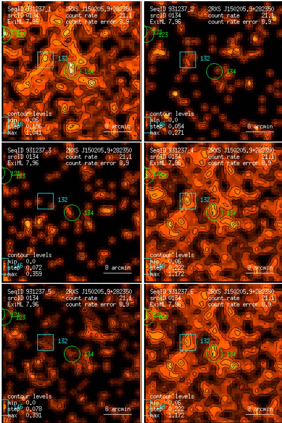
Figure 134: RASS 931237: detection 0134: band rate images, Gaussian filter: (1) PSPC channels 11 – 41, (2) 52 – 90, (3) 91 – 201, (4) 11 – 235, (5) 52 – 201, (6) 11 – 201. Broad band rates in counts/ks. Band rate contour levels in counts/ks/arcmin 2 .
