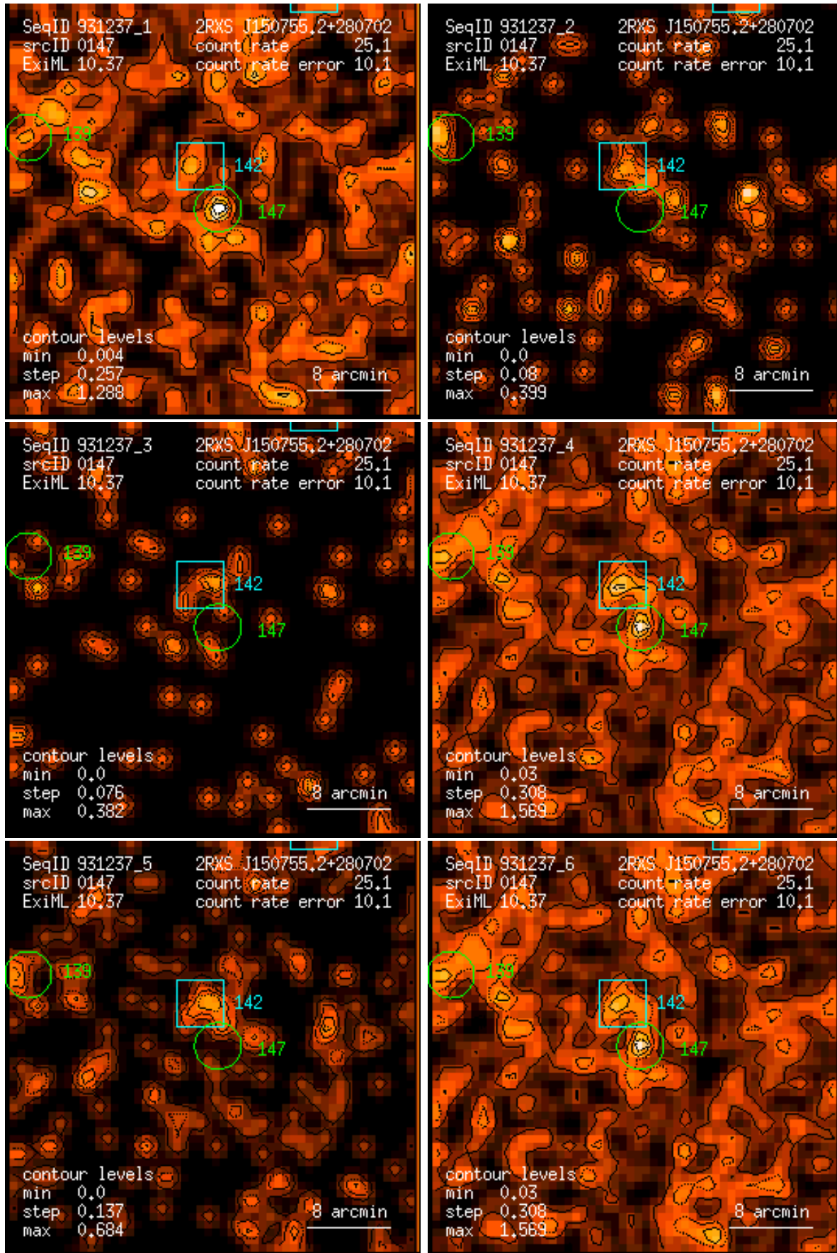
Figure 147: RASS 931237: detection 0147: band rate images, Gaussian filter: (1) PSPC channels 11 – 41, (2) 52 – 90, (3) 91 – 201, (4) 11 – 235, (5) 52 – 201, (6) 11 – 201. Broad band rates in counts/ks. Band rate contour levels in counts/ks/arcmin 2 .
