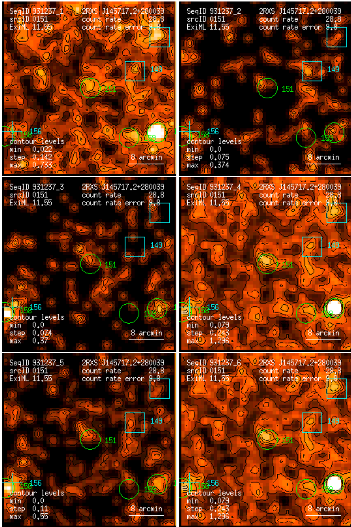
Figure 151: RASS 931237: detection 0151: band rate images, Gaussian filter: (1) PSPC channels 11 – 41, (2) 52 – 90, (3) 91 – 201, (4) 11 – 235, (5) 52 – 201, (6) 11 – 201. Broad band rates in counts/ks. Band rate contour levels in counts/ks/arcmin 2 .
