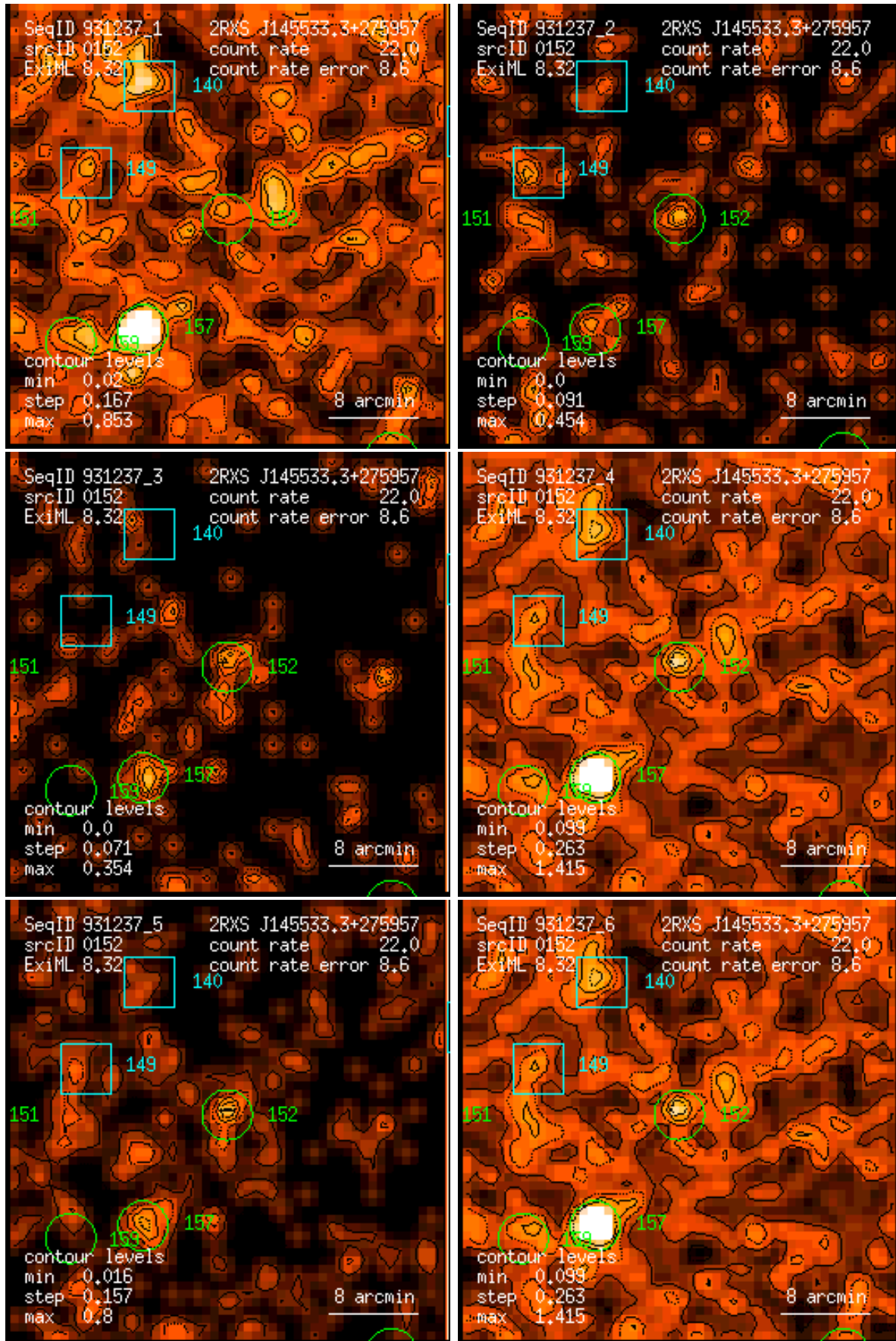
Figure 152: RASS 931237: detection 0152: band rate images, Gaussian filter: (1) PSPC channels 11 – 41, (2) 52 – 90, (3) 91 – 201, (4) 11 – 235, (5) 52 – 201, (6) 11 – 201. Broad band rates in counts/ks. Band rate contour levels in counts/ks/arcmin 2 .
