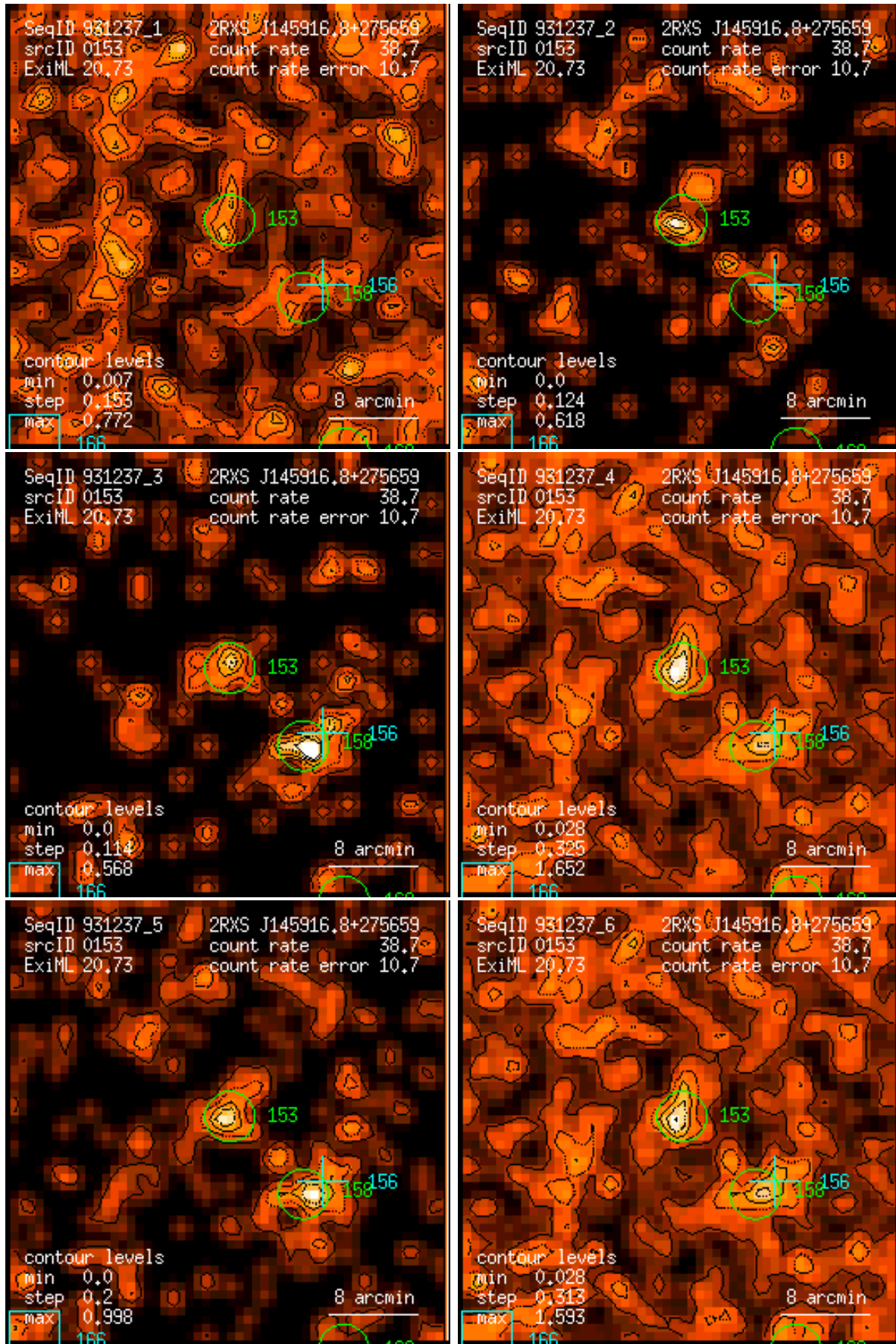
Figure 153: RASS 931237: detection 0153: band rate images, Gaussian filter: (1) PSPC channels 11 – 41, (2) 52 – 90, (3) 91 – 201, (4) 11 – 235, (5) 52 – 201, (6) 11 – 201. Broad band rates in counts/ks. Band rate contour levels in counts/ks/arcmin 2 .
