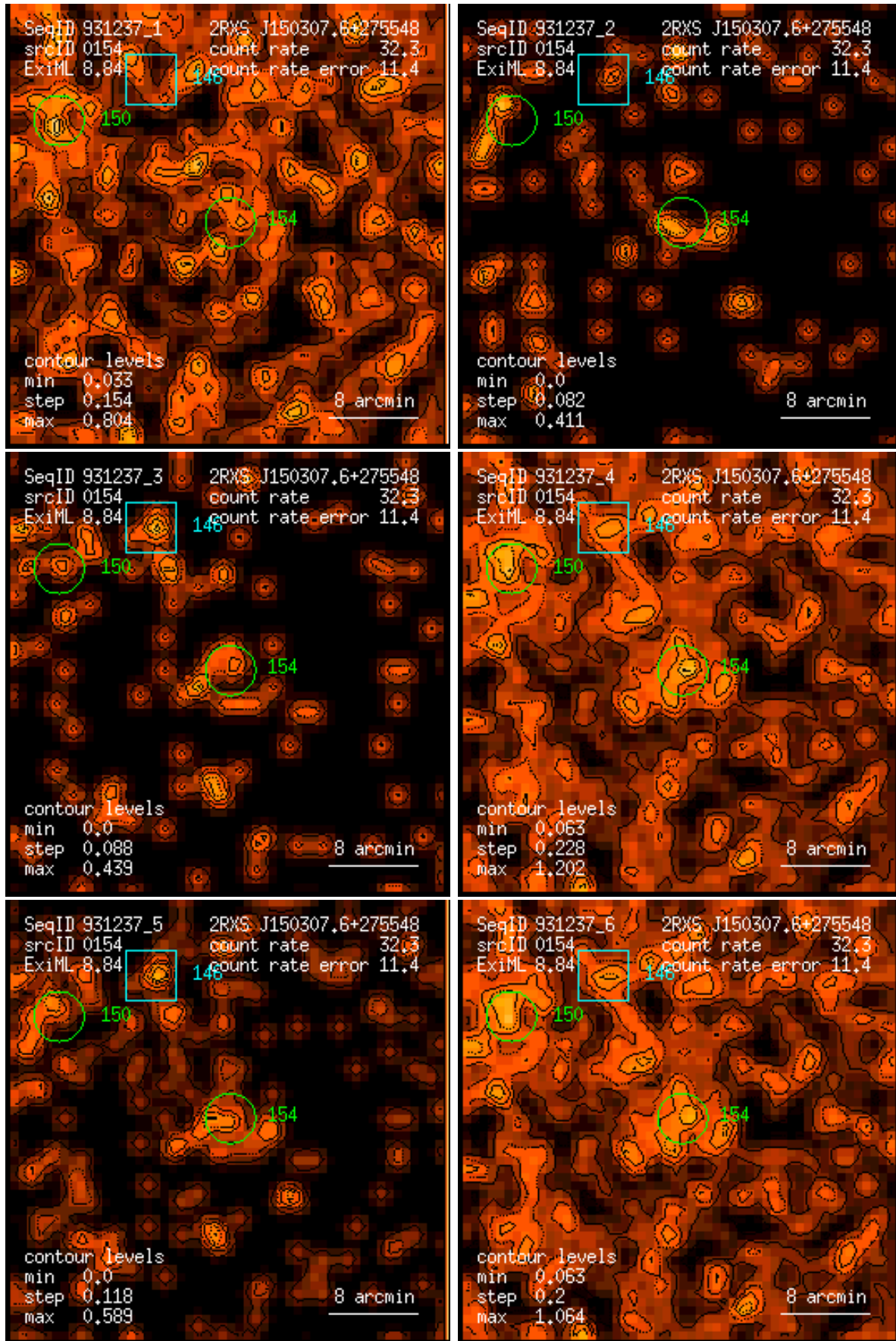
Figure 154: RASS 931237: detection 0154: band rate images, Gaussian filter: (1) PSPC channels 11 – 41, (2) 52 – 90, (3) 91 – 201, (4) 11 – 235, (5) 52 – 201, (6) 11 – 201. Broad band rates in counts/ks. Band rate contour levels in counts/ks/arcmin 2 .
