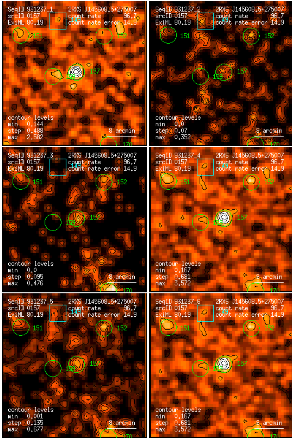
Figure 157: RASS 931237: detection 0157: band rate images, Gaussian filter: (1) PSPC channels 11 – 41, (2) 52 – 90, (3) 91 – 201, (4) 11 – 235, (5) 52 – 201, (6) 11 – 201. Broad band rates in counts/ks. Band rate contour levels in counts/ks/arcmin 2 .
