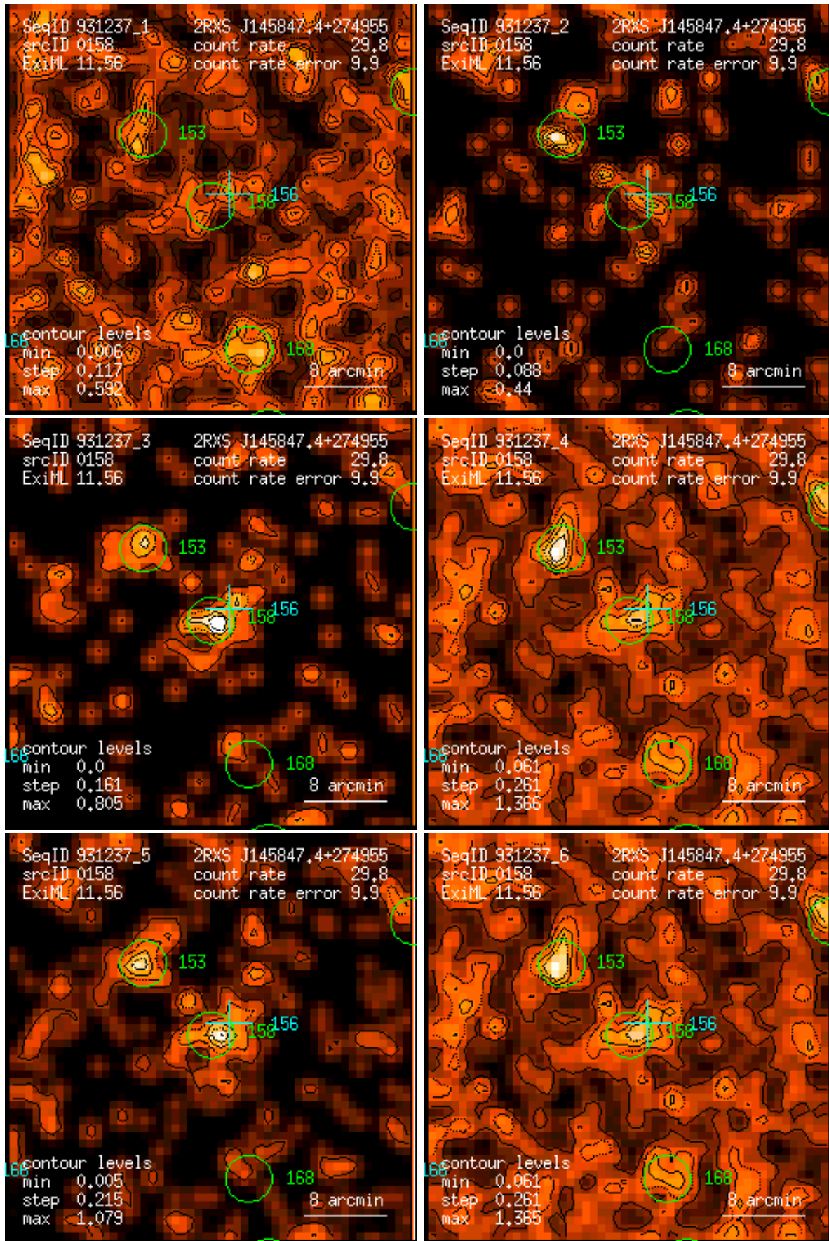
Figure 158: RASS 931237: detection 0158: band rate images, Gaussian filter: (1) PSPC channels 11 – 41, (2) 52 – 90, (3) 91 – 201, (4) 11 – 235, (5) 52 – 201, (6) 11 – 201. Broad band rates in counts/ks. Band rate contour levels in counts/ks/arcmin 2 .
