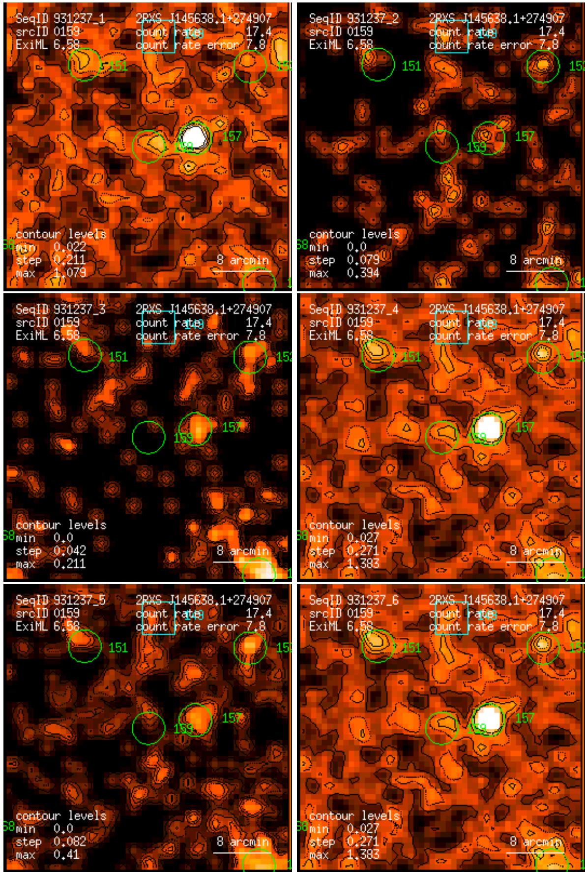
Figure 159: RASS 931237: detection 0159: band rate images, Gaussian filter: (1) PSPC channels 11 – 41, (2) 52 – 90, (3) 91 – 201, (4) 11 – 235, (5) 52 – 201, (6) 11 – 201. Broad band rates in counts/ks. Band rate contour levels in counts/ks/arcmin 2 .
