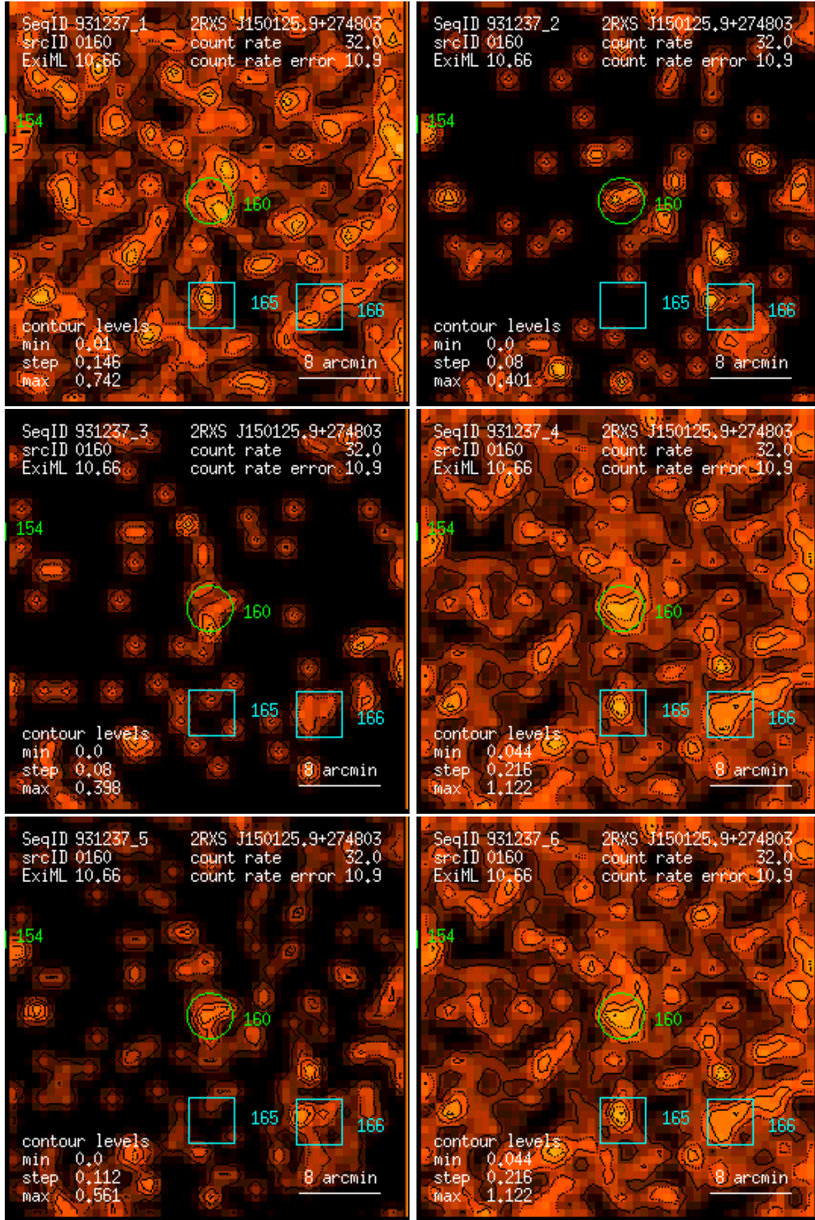
Figure 160: RASS 931237: detection 0160: band rate images, Gaussian filter: (1) PSPC channels 11 – 41, (2) 52 – 90, (3) 91 – 201, (4) 11 – 235, (5) 52 – 201, (6) 11 – 201. Broad band rates in counts/ks. Band rate contour levels in counts/ks/arcmin 2 .
