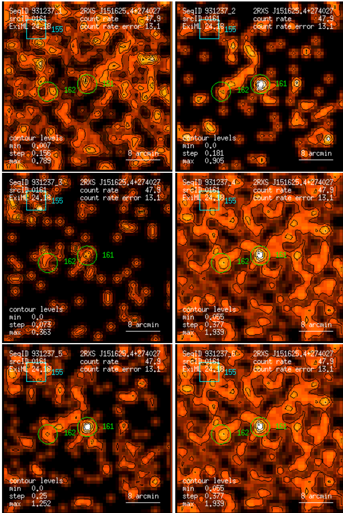
Figure 161: RASS 931237: detection 0161: band rate images, Gaussian filter: (1) PSPC channels 11 – 41, (2) 52 – 90, (3) 91 – 201, (4) 11 – 235, (5) 52 – 201, (6) 11 – 201. Broad band rates in counts/ks. Band rate contour levels in counts/ks/arcmin 2 .
