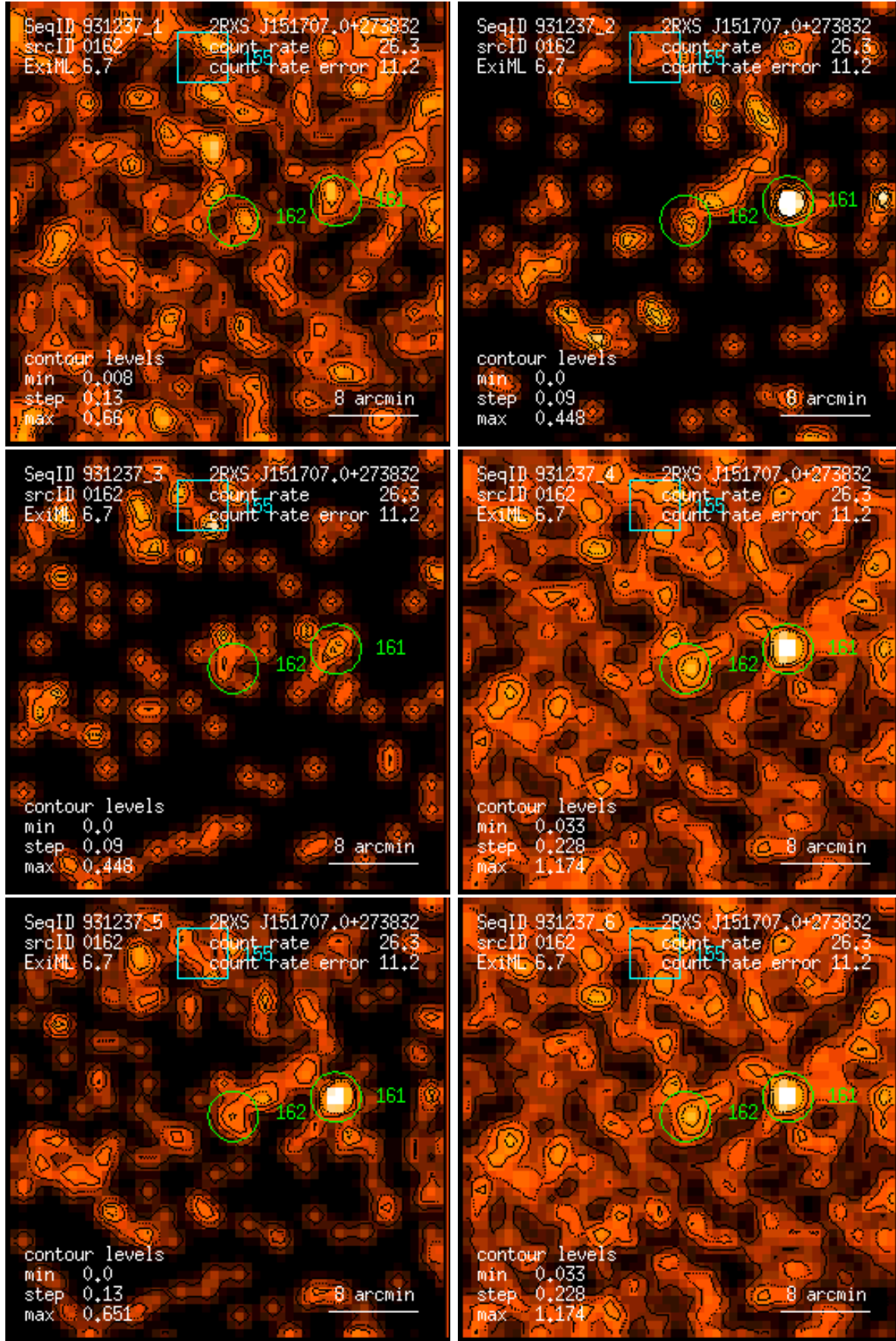
Figure 162: RASS 931237: detection 0162: band rate images, Gaussian filter: (1) PSPC channels 11 – 41, (2) 52 – 90, (3) 91 – 201, (4) 11 – 235, (5) 52 – 201, (6) 11 – 201. Broad band rates in counts/ks. Band rate contour levels in counts/ks/arcmin 2 .
