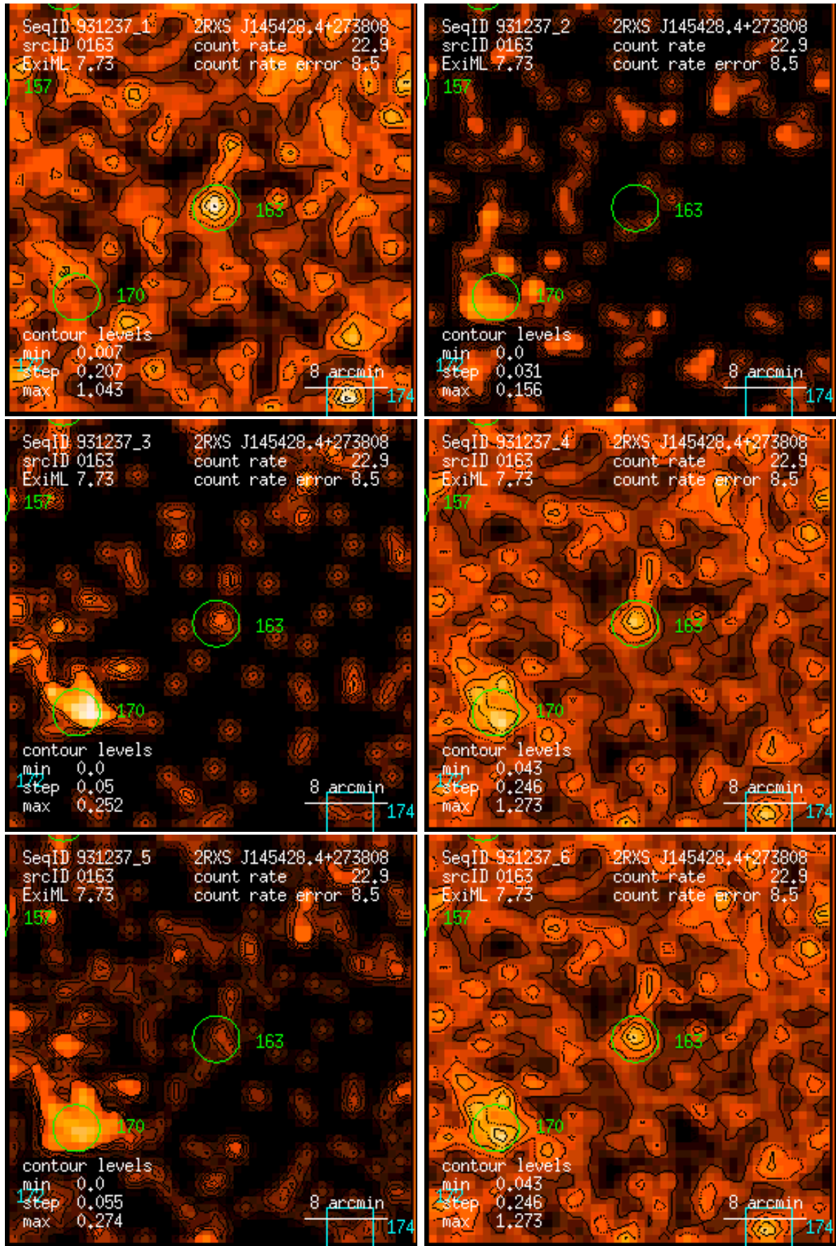
Figure 163: RASS 931237: detection 0163: band rate images, Gaussian filter: (1) PSPC channels 11 – 41, (2) 52 – 90, (3) 91 – 201, (4) 11 – 235, (5) 52 – 201, (6) 11 – 201. Broad band rates in counts/ks. Band rate contour levels in counts/ks/arcmin 2 .
