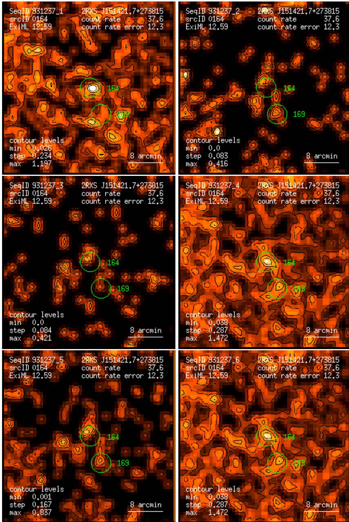
Figure 164: RASS 931237: detection 0164: band rate images, Gaussian filter: (1) PSPC channels 11 – 41, (2) 52 – 90, (3) 91 – 201, (4) 11 – 235, (5) 52 – 201, (6) 11 – 201. Broad band rates in counts/ks. Band rate contour levels in counts/ks/arcmin 2 .
