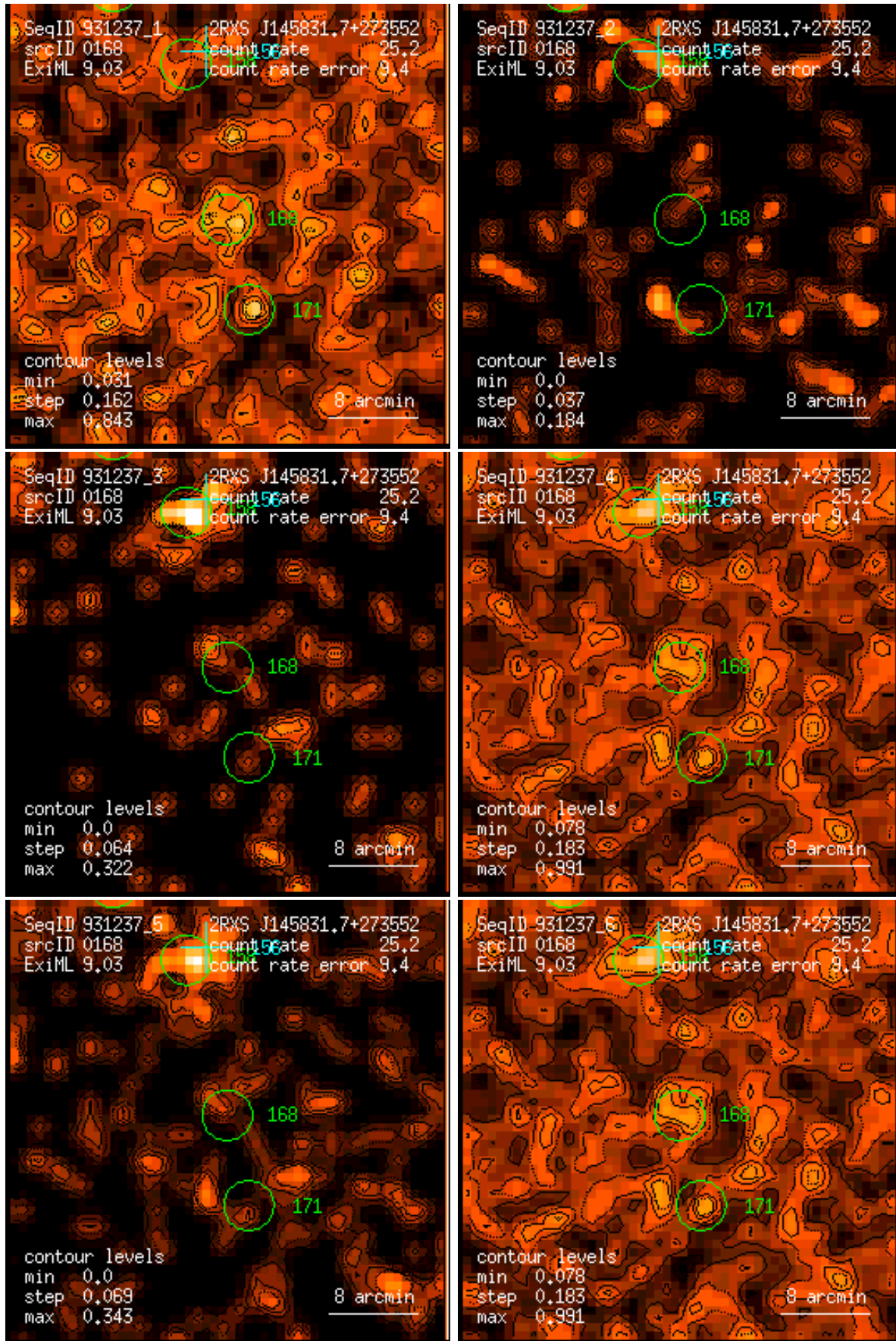
Figure 168: RASS 931237: detection 0168: band rate images, Gaussian filter: (1) PSPC channels 11 – 41, (2) 52 – 90, (3) 91 – 201, (4) 11 – 235, (5) 52 – 201, (6) 11 – 201. Broad band rates in counts/ks. Band rate contour levels in counts/ks/arcmin 2 .
