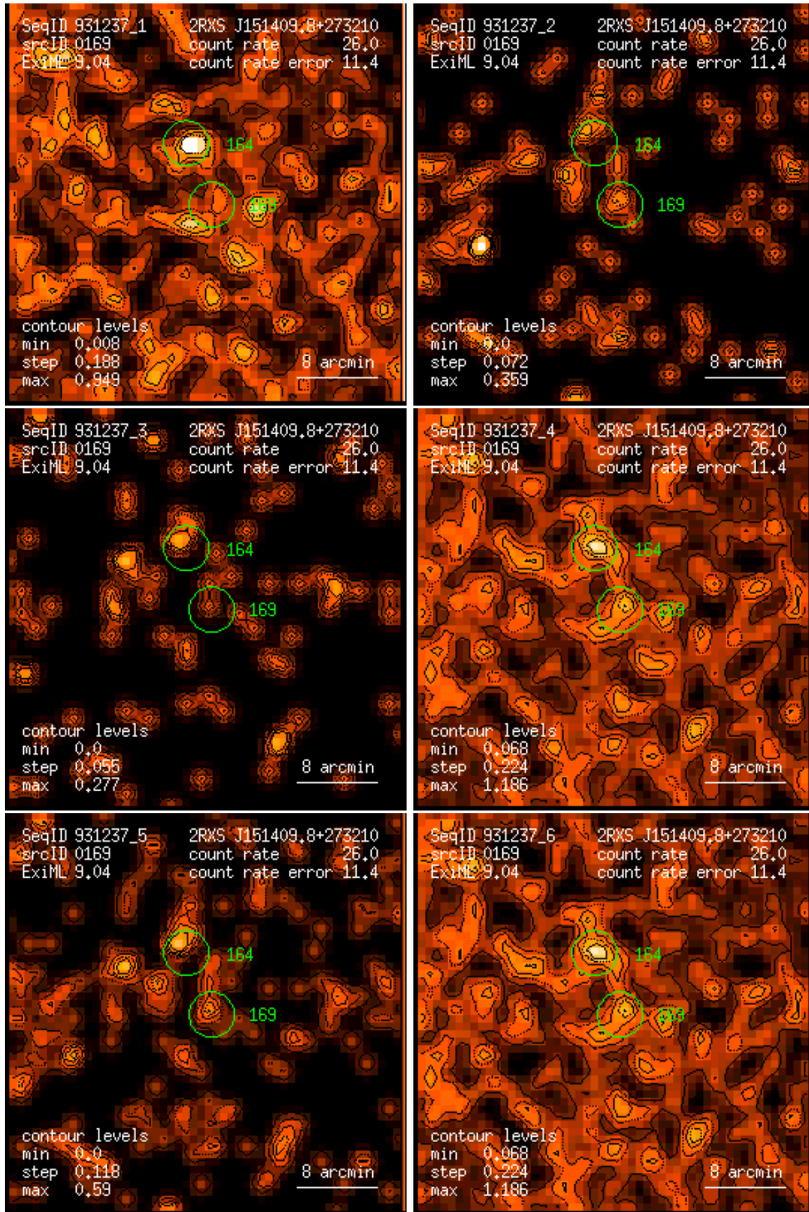
Figure 169: RASS 931237: detection 0169: band rate images, Gaussian filter: (1) PSPC channels 11 – 41, (2) 52 – 90, (3) 91 – 201, (4) 11 – 235, (5) 52 – 201, (6) 11 – 201. Broad band rates in counts/ks. Band rate contour levels in counts/ks/arcmin 2 .
