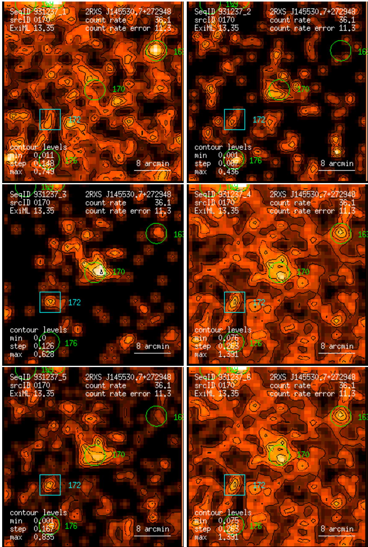
Figure 170: RASS 931237: detection 0170: band rate images, Gaussian filter: (1) PSPC channels 11 – 41, (2) 52 – 90, (3) 91 – 201, (4) 11 – 235, (5) 52 – 201, (6) 11 – 201. Broad band rates in counts/ks. Band rate contour levels in counts/ks/arcmin 2 .
