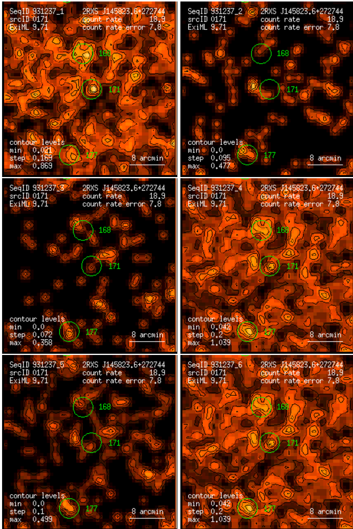
Figure 171: RASS 931237: detection 0171: band rate images, Gaussian filter: (1) PSPC channels 11 – 41, (2) 52 – 90, (3) 91 – 201, (4) 11 – 235, (5) 52 – 201, (6) 11 – 201. Broad band rates in counts/ks. Band rate contour levels in counts/ks/arcmin 2 .
