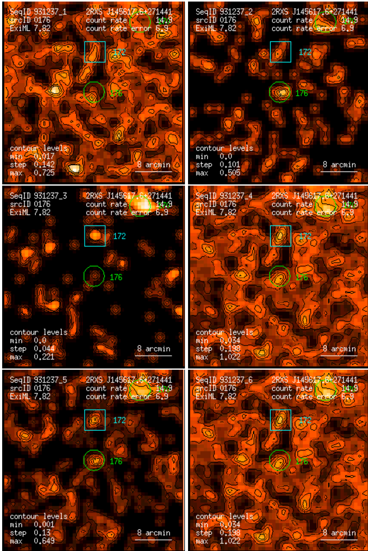
Figure 176: RASS 931237: detection 0176: band rate images, Gaussian filter: (1) PSPC channels 11 – 41, (2) 52 – 90, (3) 91 – 201, (4) 11 – 235, (5) 52 – 201, (6) 11 – 201. Broad band rates in counts/ks. Band rate contour levels in counts/ks/arcmin 2 .
