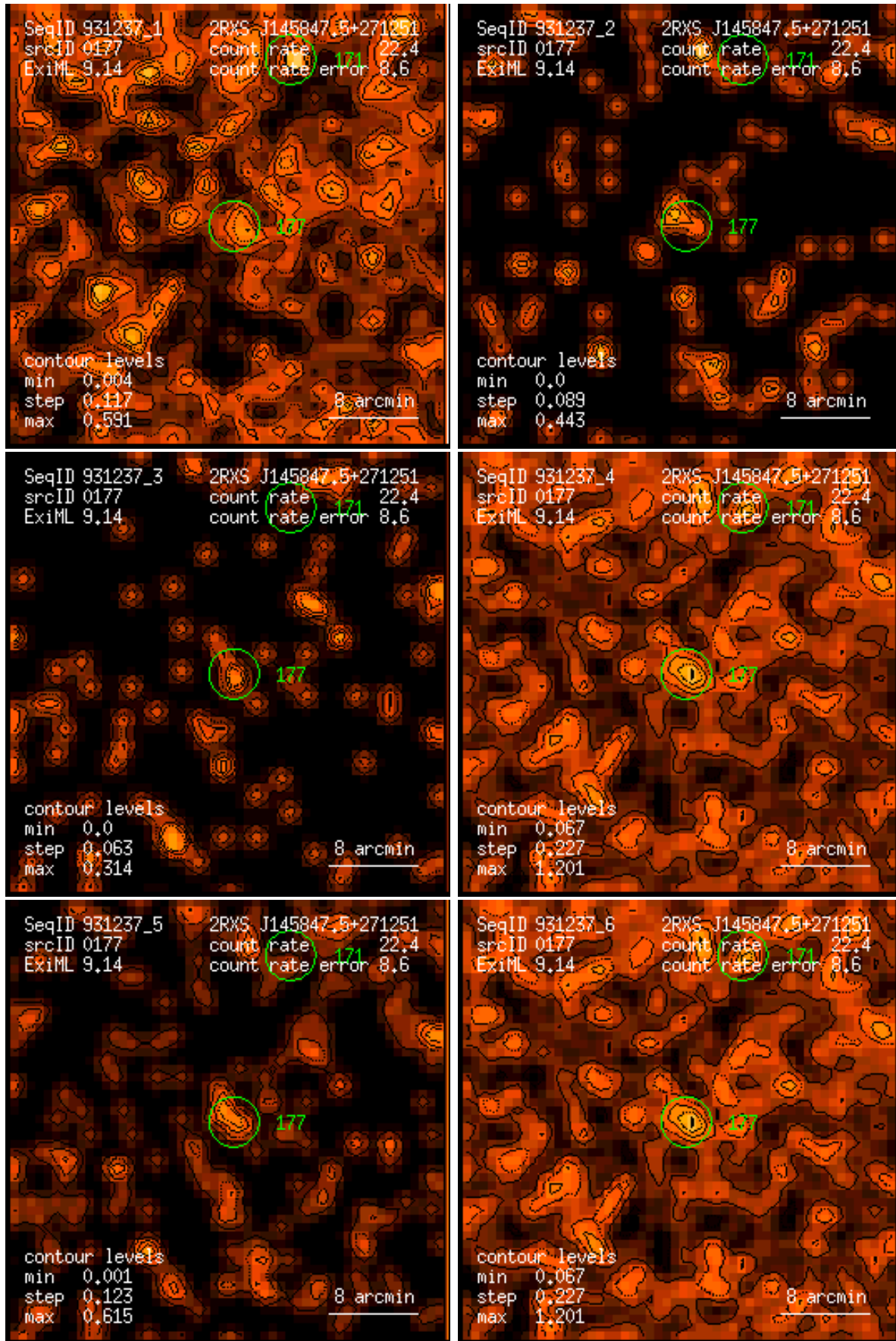
Figure 177: RASS 931237: detection 0177: band rate images, Gaussian filter: (1) PSPC channels 11 – 41, (2) 52 – 90, (3) 91 – 201, (4) 11 – 235, (5) 52 – 201, (6) 11 – 201. Broad band rates in counts/ks. Band rate contour levels in counts/ks/arcmin 2 .
