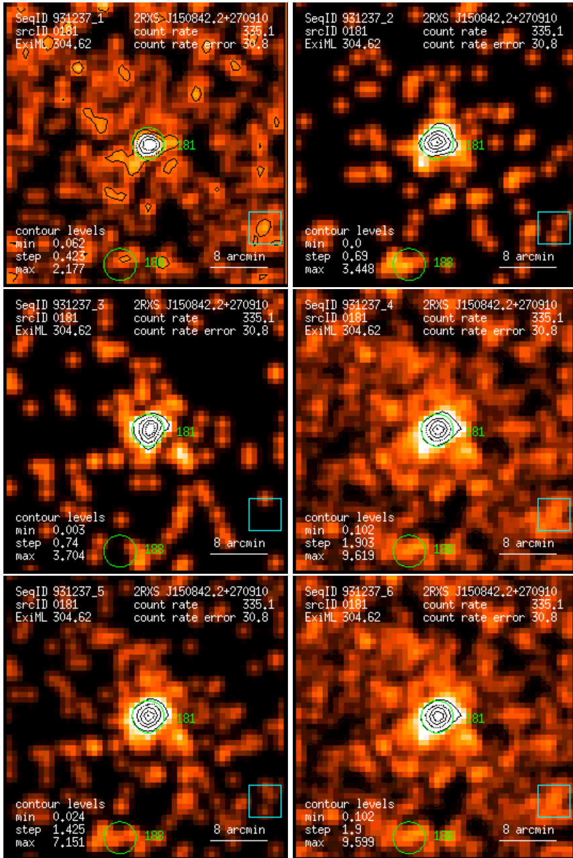
Figure 181: RASS 931237: detection 0181: band rate images, Gaussian filter: (1) PSPC channels 11 – 41, (2) 52 – 90, (3) 91 – 201, (4) 11 – 235, (5) 52 – 201, (6) 11 – 201. Broad band rates in counts/ks. Band rate contour levels in counts/ks/arcmin 2 .
