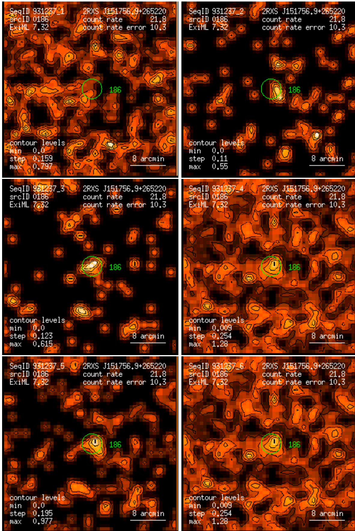
Figure 186: RASS 931237: detection 0186: band rate images, Gaussian filter: (1) PSPC channels 11 – 41, (2) 52 – 90, (3) 91 – 201, (4) 11 – 235, (5) 52 – 201, (6) 11 – 201. Broad band rates in counts/ks. Band rate contour levels in counts/ks/arcmin 2 .
