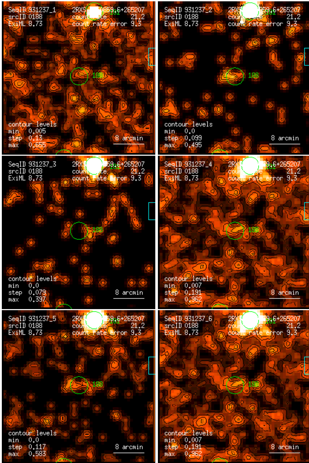
Figure 188: RASS 931237: detection 0188: band rate images, Gaussian filter: (1) PSPC channels 11 – 41, (2) 52 – 90, (3) 91 – 201, (4) 11 – 235, (5) 52 – 201, (6) 11 – 201. Broad band rates in counts/ks. Band rate contour levels in counts/ks/arcmin 2 .
