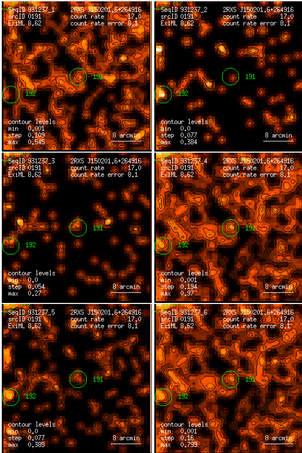
Figure 191: RASS 931237: detection 0191: band rate images, Gaussian filter: (1) PSPC channels 11 – 41, (2) 52 – 90, (3) 91 – 201, (4) 11 – 235, (5) 52 – 201, (6) 11 – 201. Broad band rates in counts/ks. Band rate contour levels in counts/ks/arcmin 2 .
